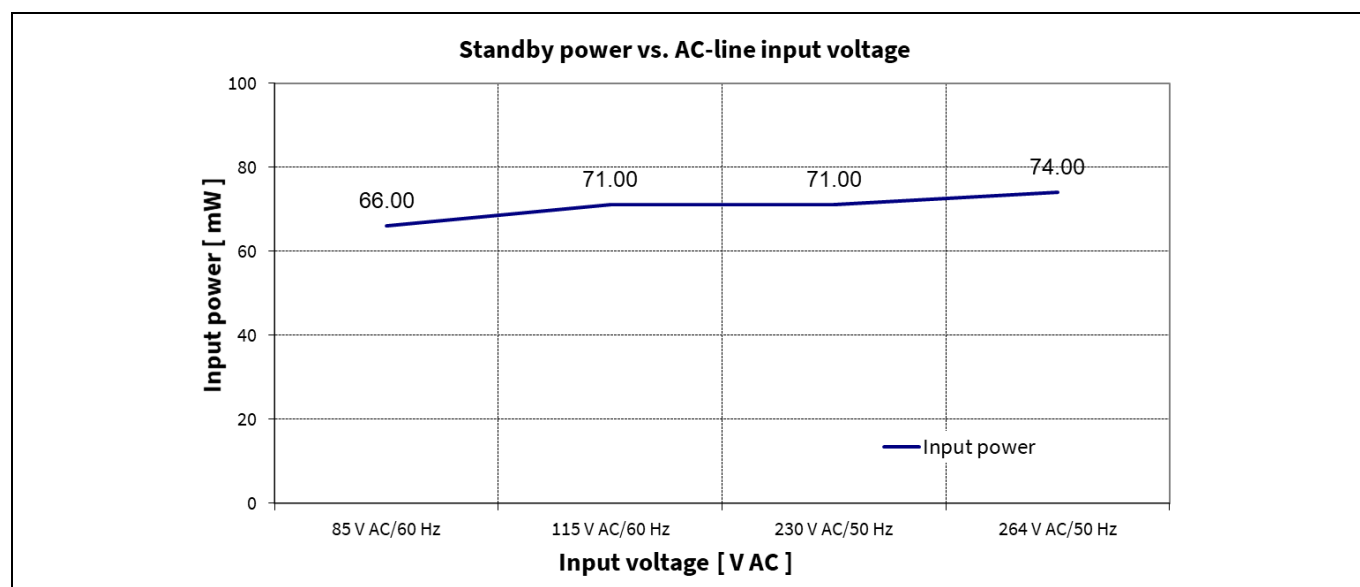
Figure 7 Standby power at 10 k \Omega R9 (22 mW) vs. AC line input voltage. Bleeder resistor (R9) prevents the output voltage from increasing during no-load conditions.
