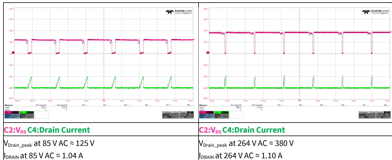
Figure 14 Drain voltage and current at maximum load
