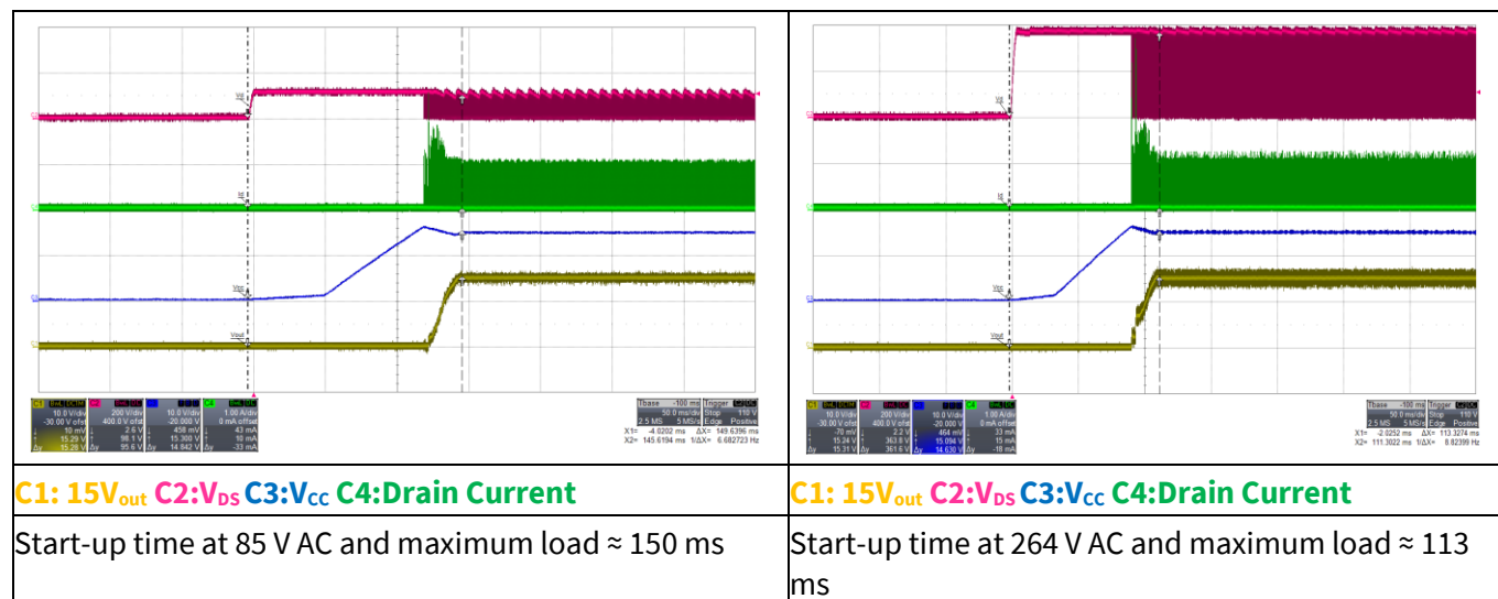
Figure 12 Start-up
