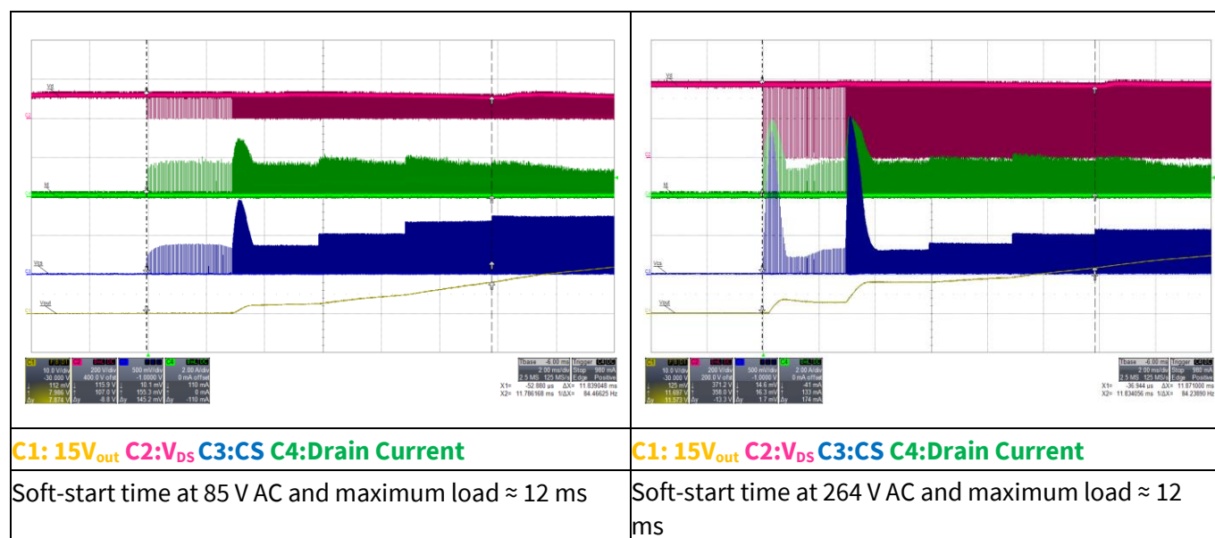
Figure 13 Soft-start
