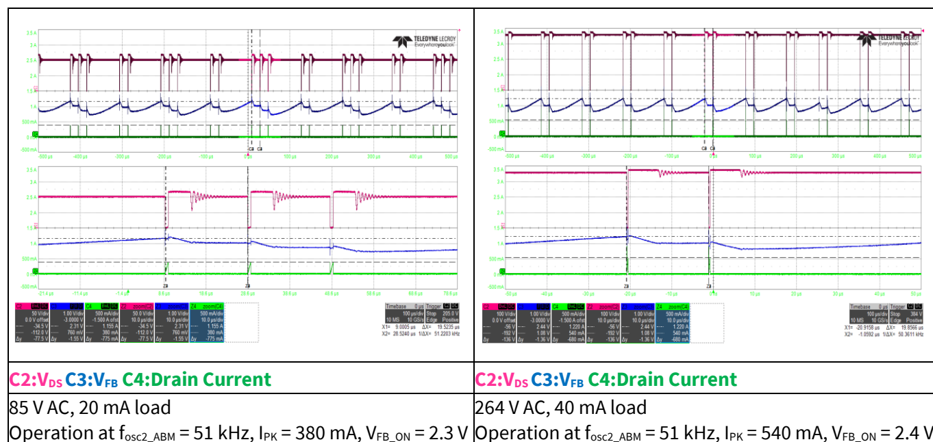
Figure 16 ABM operation
