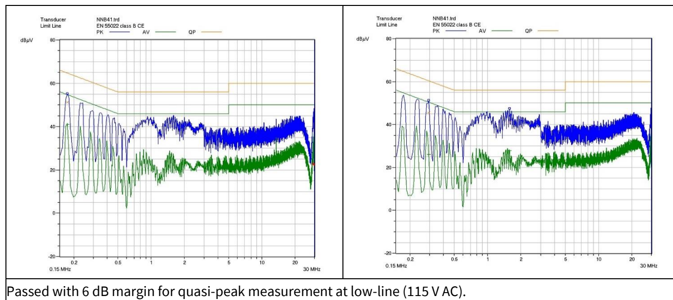
Figure 9 Conducted emissions at 115 V AC with full load
