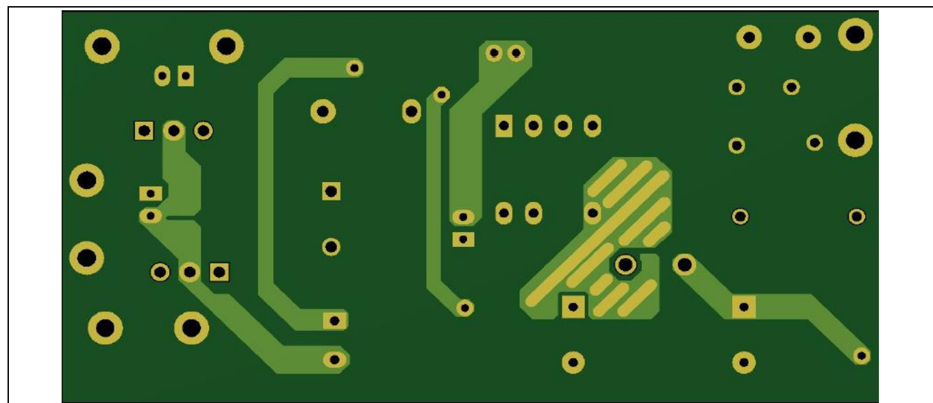
Figure 5 Bottom-side copper
