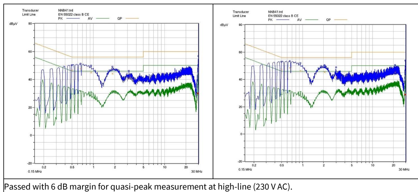
Figure 10 Conducted emissions at 230 V AC with full load
