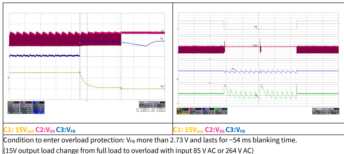
Figure 17 Overload protection
