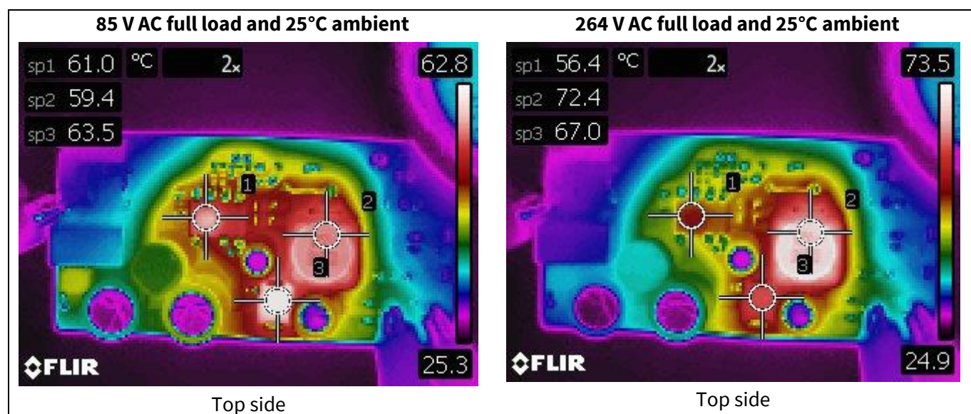
Figure 11 Infrared thermal image of EVAL_5BR4780BZ-1_450mA1
