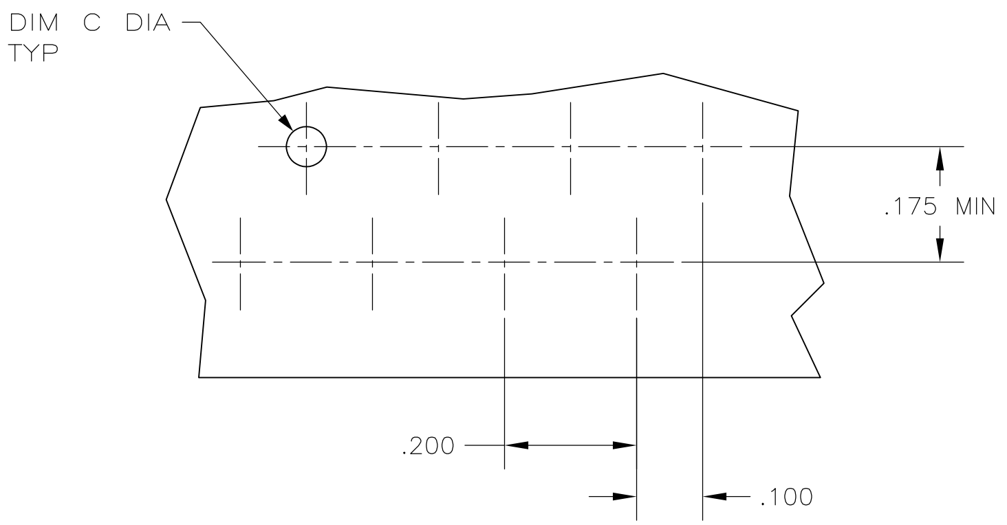
SUGGESTED PRINTED CIRCUIT BOARD MOUNTING DIMENSIONS
