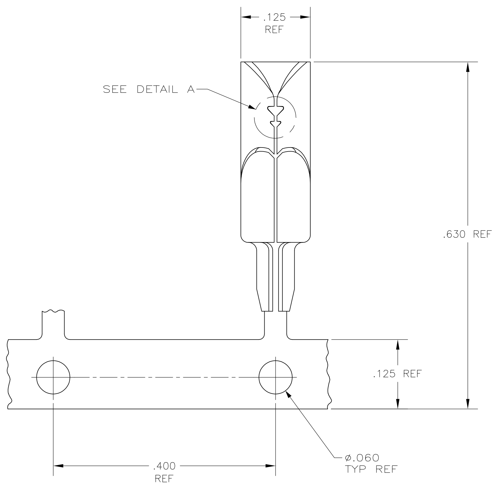
STRIP MOUNTED -2, -5 & -7 ONLY
