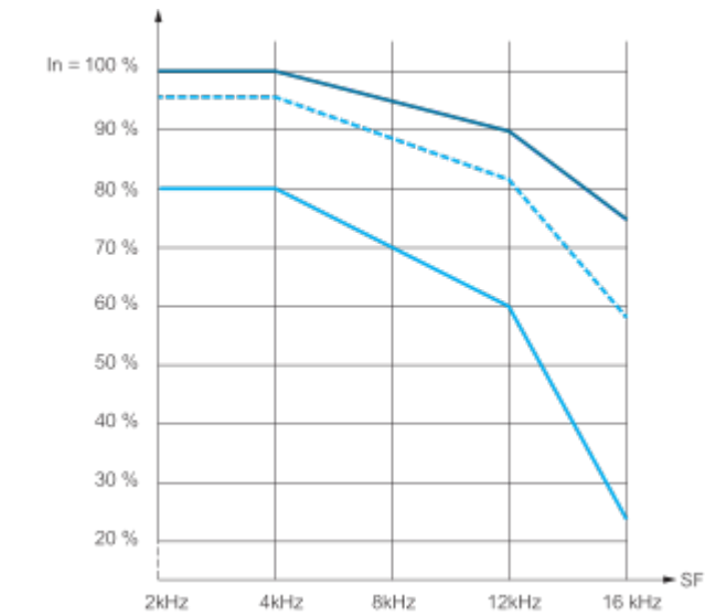
— 40 °C (104 °F) - Mounting type B - - - 50 °C (122 °F) - Mounting type B — 60 °C (140 °F) - Mounting type B In : Nominal Drive Current SF : Switching Frequency
