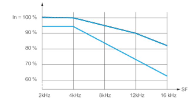
— 40 °C (104 °F) - Mounting type B - - - 50 °C (122 °F) - Mounting type B — 60 °C (140 °F) - Mounting type B In : Nominal Drive Current SF : Switching Frequency
