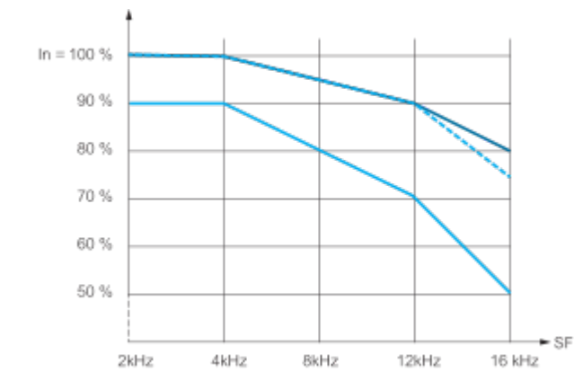
— 40 °C (104 °F) - Mounting type A - - - 50 °C (122 °F) - Mounting type A — 60 °C (140 °F) - Mounting type A In : Nominal Drive Current SF : Switching Frequency
