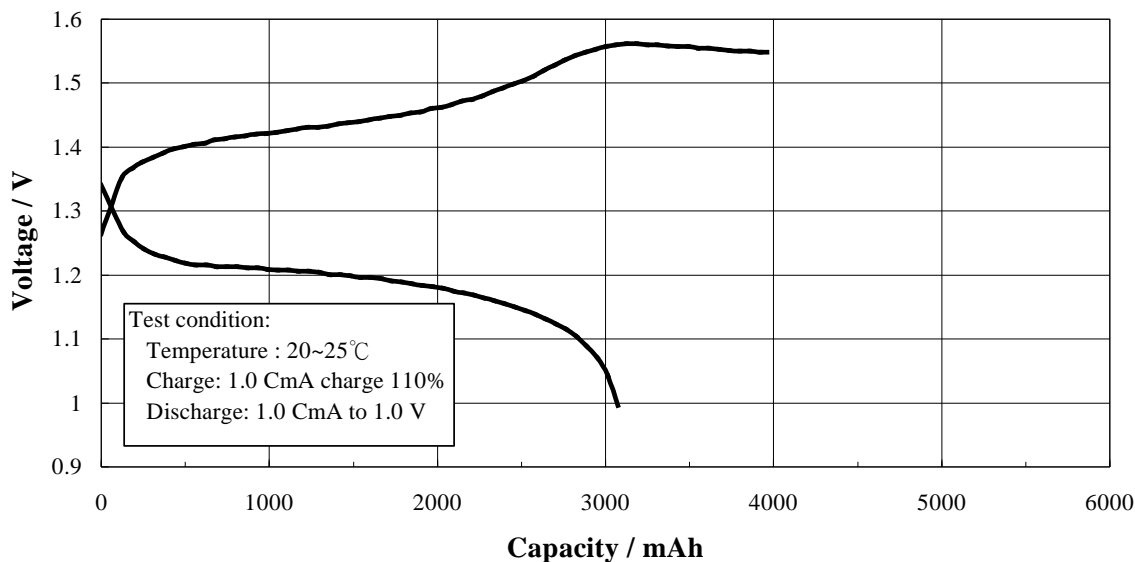
Battery 4/3A High Rate Charge/Discharge Voltage Characteristics
