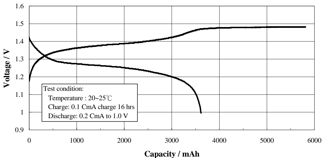
Battery 4/3A Standard Charge/Discharge Voltage Characteristics
