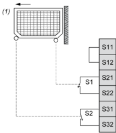
(1) Protective guard
