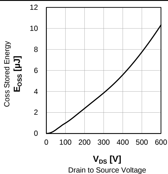
Fig.16 Typ. Coss Stored Energy
