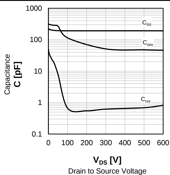
Fig.15 Typ. Capacitance
