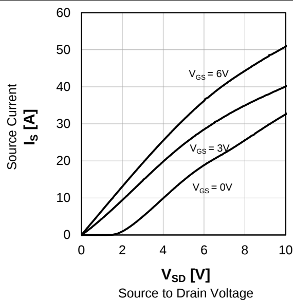
Fig.14 Channel Reverse Characteristics
