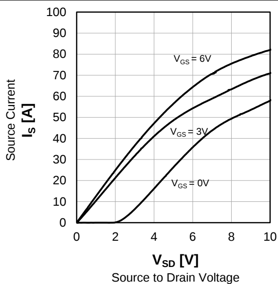
Fig.13 Channel Reverse Characteristics
