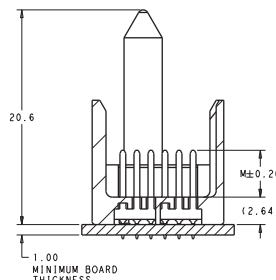
Section Z-Z
