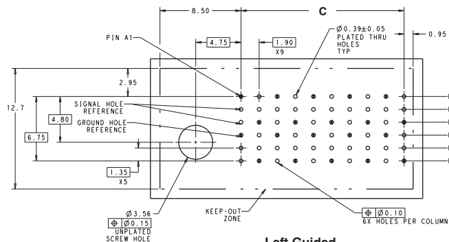
Left Guided Backplane Hole Pattern (Connector Side)
