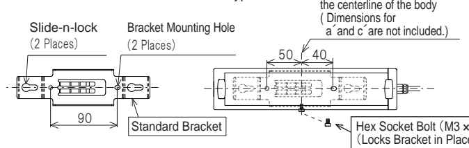
Figure 1. AG Type Installation -1
