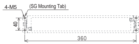
Figure 8. SG Type Mounting Hole Dimensions
