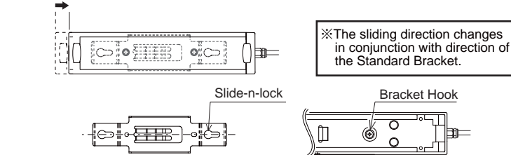
Figure 4. AG Type Slide Installation -1
