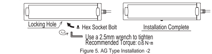
Figure 5. AG Type Installation -2
