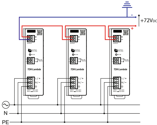
Fig. 29: Connection scheme for series operation with positive voltage level
