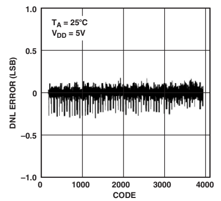
TPC 6. AD5322 Typical DNL Plot
