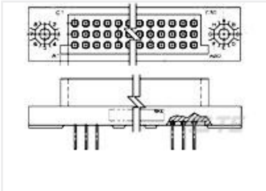
TE Part #443857-3 3 ROW BOX RECEPTACLE, 180 POS
