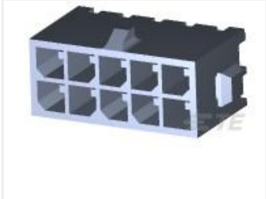
TE Part #4-794630-0 10POS MICRO MNL ASSY,VRT,HDR
