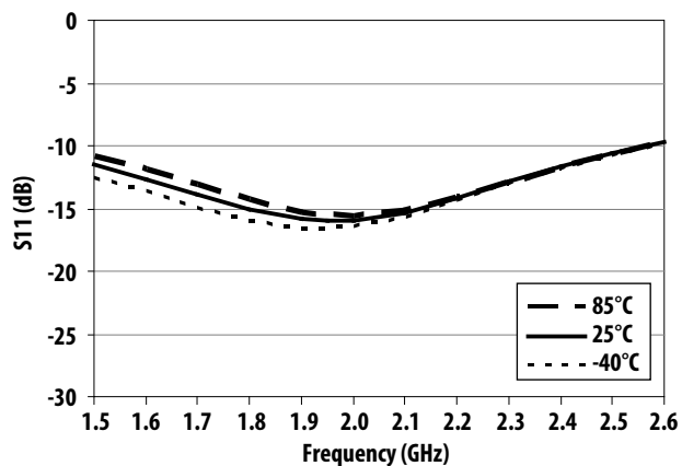
Figure 26. S11 over Frequency and Temperature
