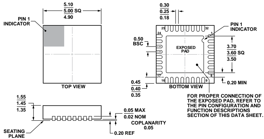
Figure 40. 32-Lead Lead Frame Chip Scale Package [LFCSP_LQ] 5 mm x 5 mm Body, Thick Quad (CP-32-17) Dimensions shown in millimeters
