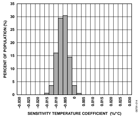
Figure 14. Z-Axis Sensitivity Temperature Coefficient, V_S = V_{DD/IO} = 3.3 V
