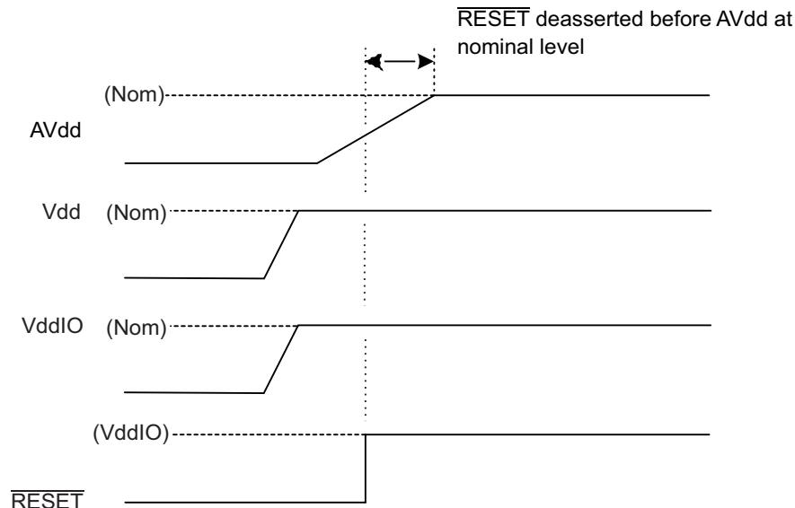
FIGURE 5-2: POWER SEQUENCING ON THE ATMXT336UD – LATE RISE ON AVDD
