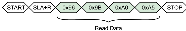
FIGURE 7-6: EXAMPLE OF A FOUR-BYTE READ – ENCRYPTION ACTIVE
