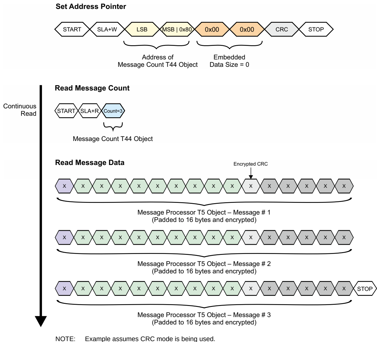
FIGURE 7-11: EXAMPLE READ FROM MESSAGE PROCESSOR T5 – ENCRYPTION ACTIVE
