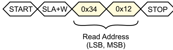
FIGURE 7-5: EXAMPLE OF A FOUR-BYTE READ – ENCRYPTION NOT ACTIVE
