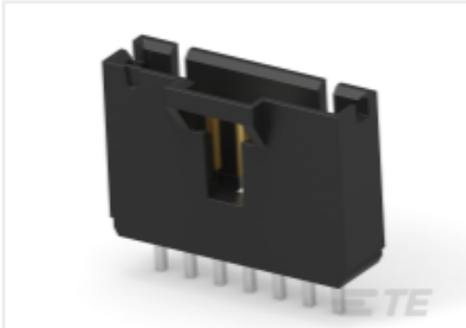
TE Part # 5-104362-6 07 MTE HDR SRST LATCH W/HLDWN
