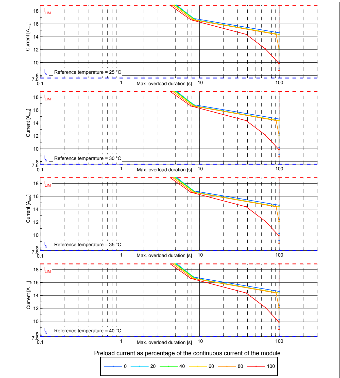
Figure 2: 8BVI0055HWSS.000-x - Overload characteristics, overload response - ERROR+STOP
