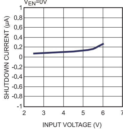
Shutdown Current vs. Input Voltage V_{EN} = 0V
