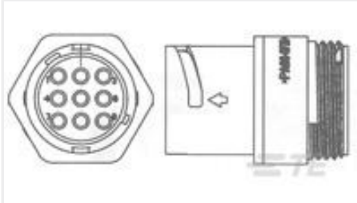
TE Part #1445828-1 REC, 11-6, FRE HNG, SM INS, STD KE
