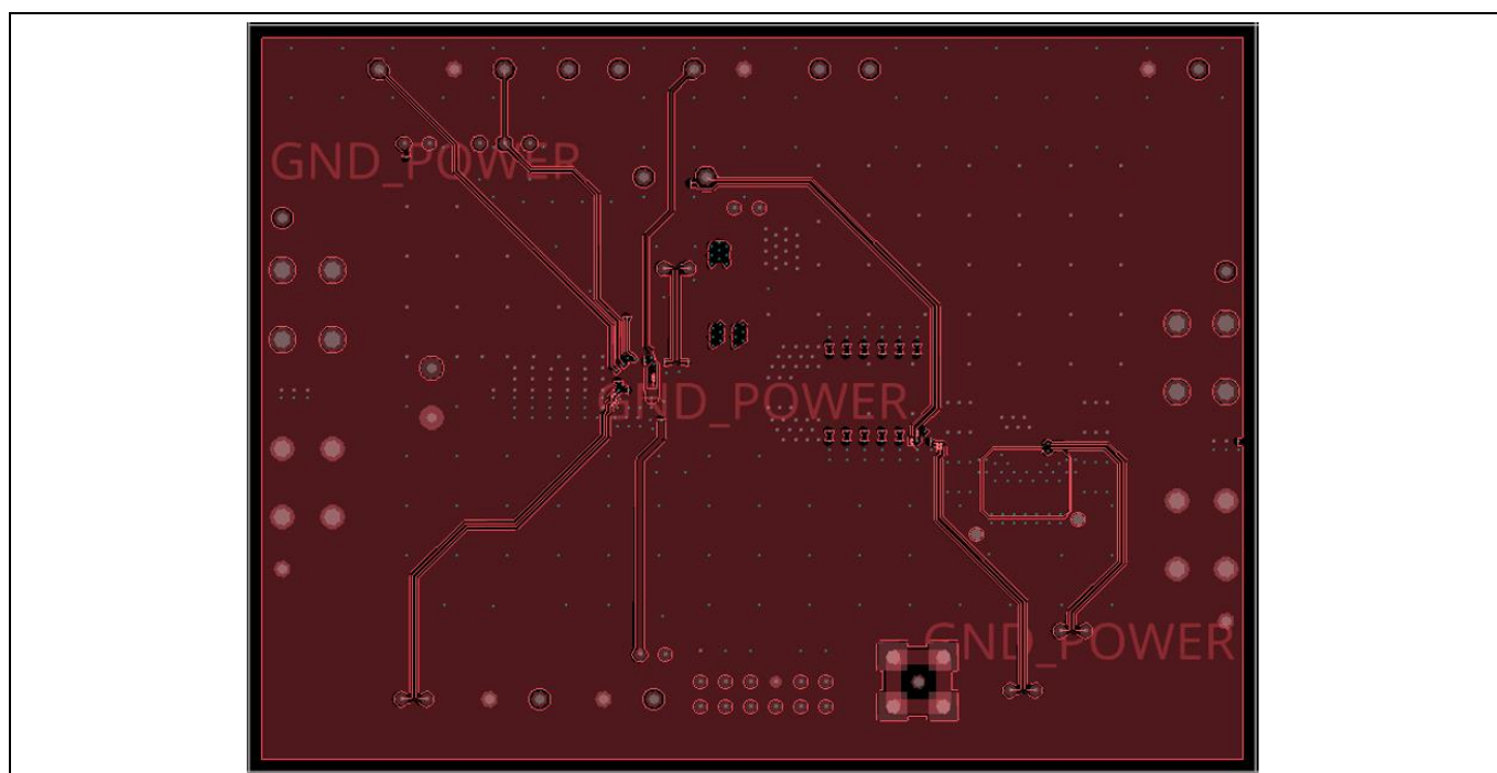
Figure 5 Inner layer2
