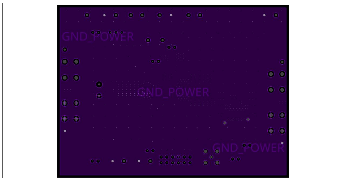
Figure 4 Inner layer 1
