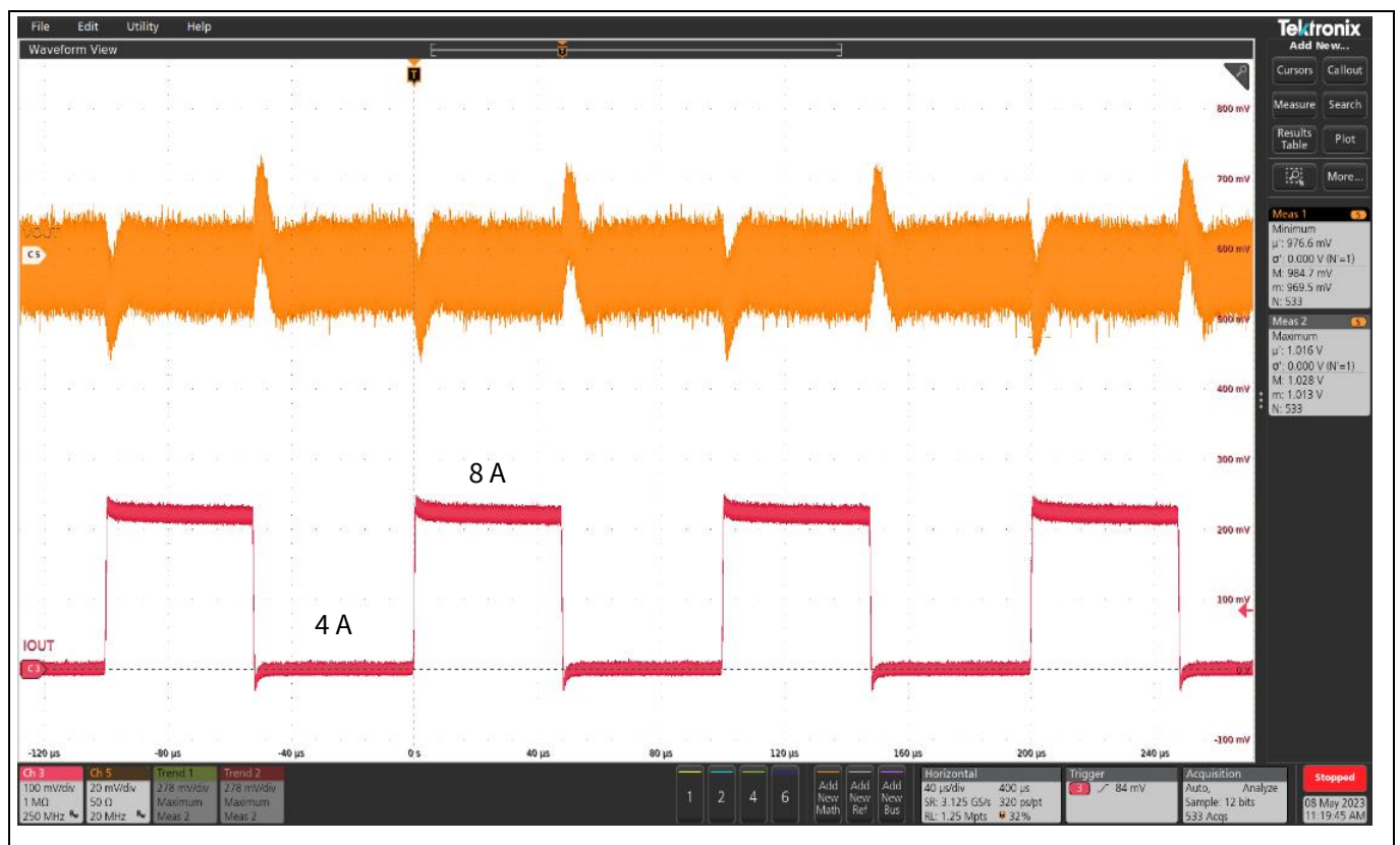
Figure 17 Transient response at 4 A step load current at 10 A/μs slew rate: I_{OUT} = 4\text{ A} - 8\text{ A} , (Ch5: V_{OUT} , Ch3: I_{OUT} ), pk-pk: 39.4 mV, F_{SW} = 800\text{ kHz}
