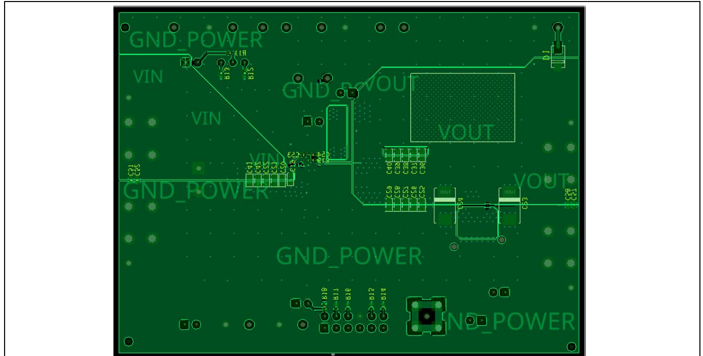
Figure 3 Bottom layer
