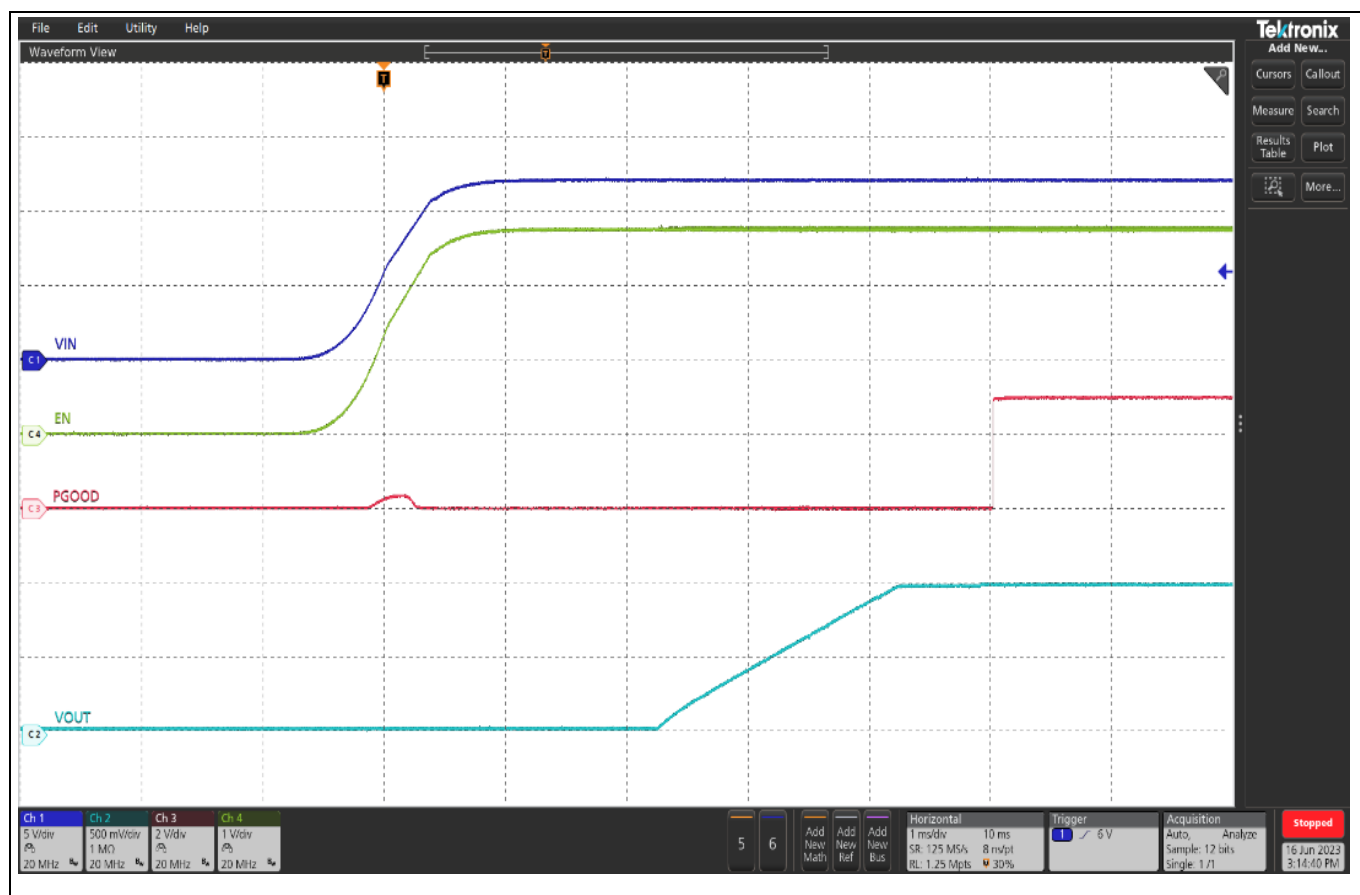
Figure 11 Start-up at 12 A load, (Ch1: V_{IN} , Ch2: V_{OUT} , Ch3: P_{GOOD} , Ch4: enable)
