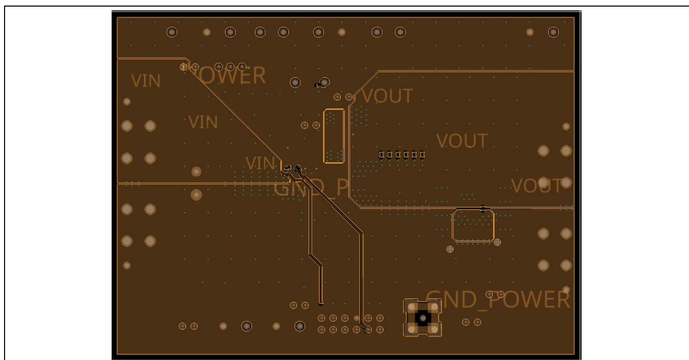
Figure 6 Inner layer 3
