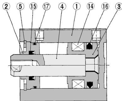
Rod end male thread
