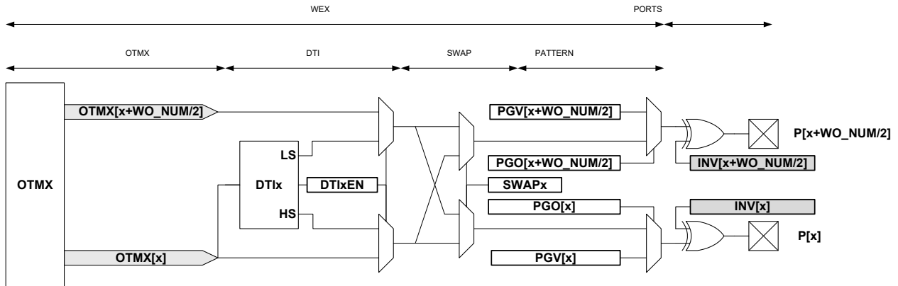
Figure 35-36. Waveform Extension Stage Details
