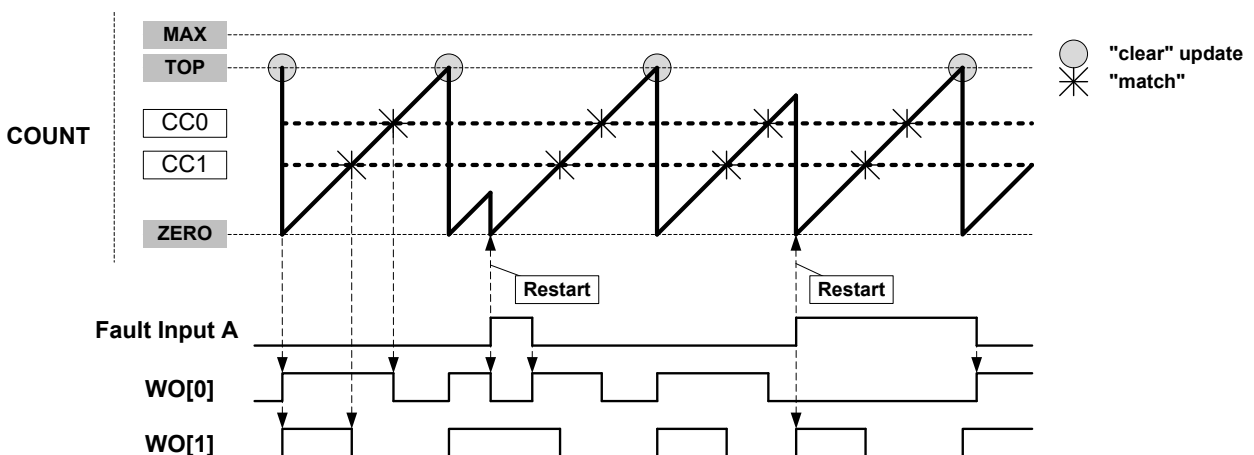
Figure 35-28. Waveform Generation in RAMP1 mode with Restart Action
