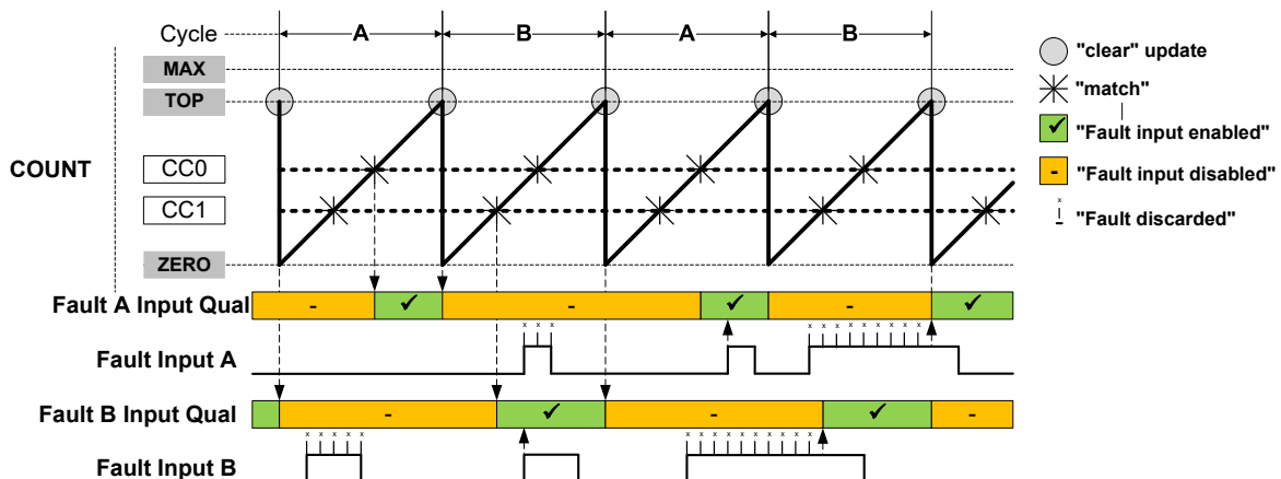
Figure 35-26. Fault Qualification in RAMP2 Operation
