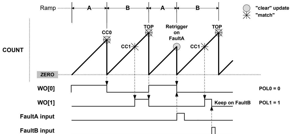
Figure 35-22. Critical RAMP2 Operation With 2 Channels
