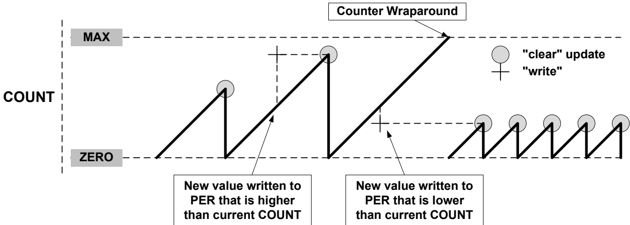
Figure 35-11. Unbuffered Single-Slope Up-Counting Operation
