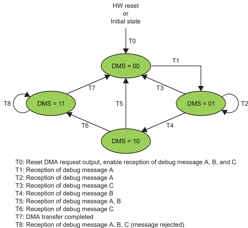
Figure 33-9. Debug Message Handling State Machine
