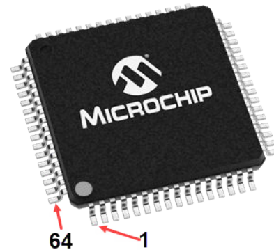
Figure 4-5. TQFP
