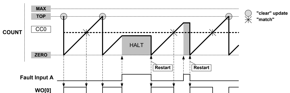
Figure 35-32. Waveform Generation with Halt and Restart Actions
