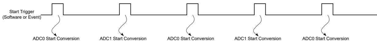
Figure 37-10. Interleaved Dual-Mode Trigger Selection
