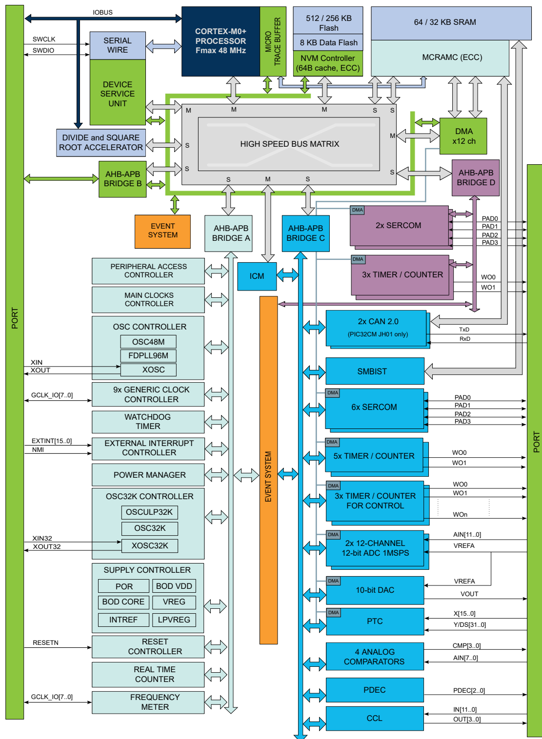
Figure 3-1. PIC32CM JH00/JH01 Block Diagram
