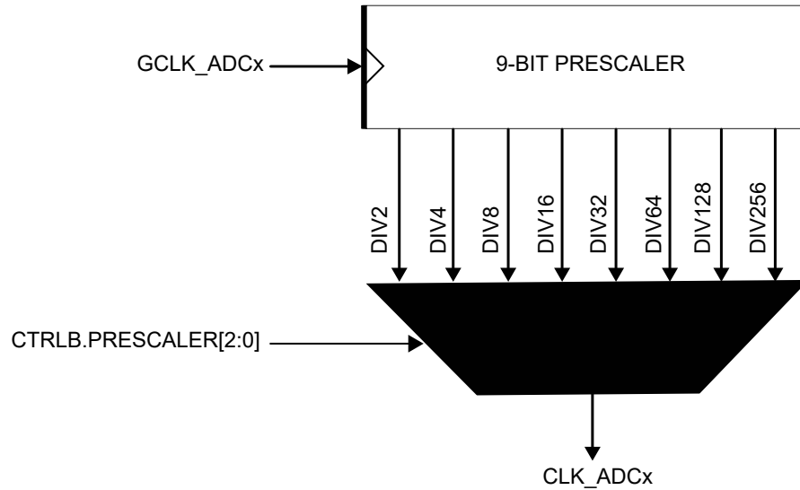
Figure 37-2. ADC Prescaler
