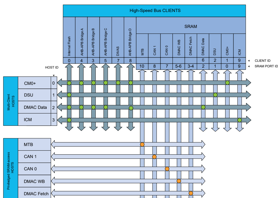
Figure 11-1. Host-Client Relation High-Speed Bus Matrix
