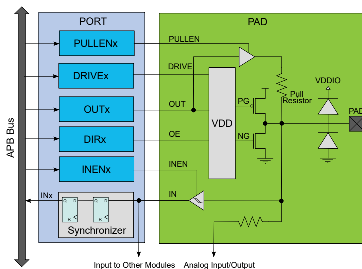
Figure 27-2. Overview of the PORT
