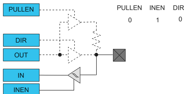
Figure 27-4. I/O configuration - Standard Input
