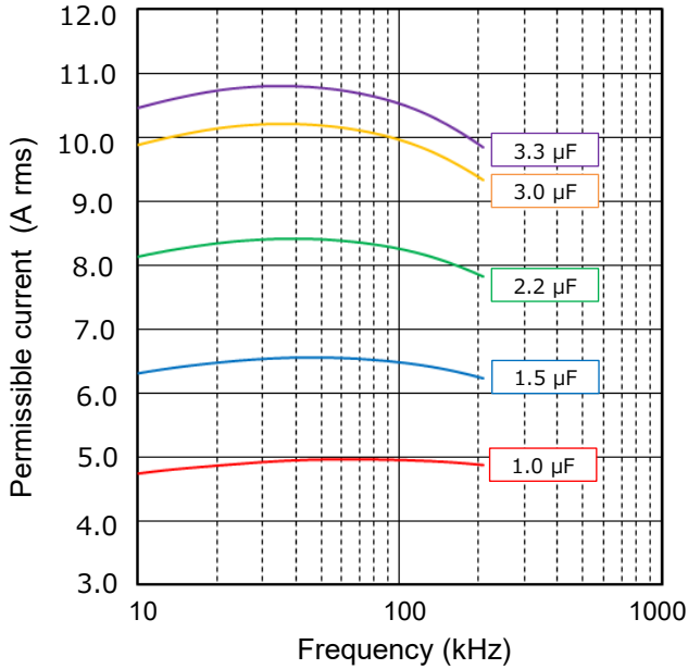
[ Permissible Current ]
