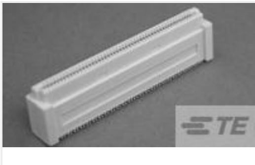
TE Part #5084618-2 0.8FH,R13H.5,060,30/Sn,TR,SC
