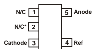
ZTL431_E5 SOT235 (Top View)
