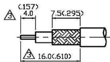
STRIPPING DIMENSION
