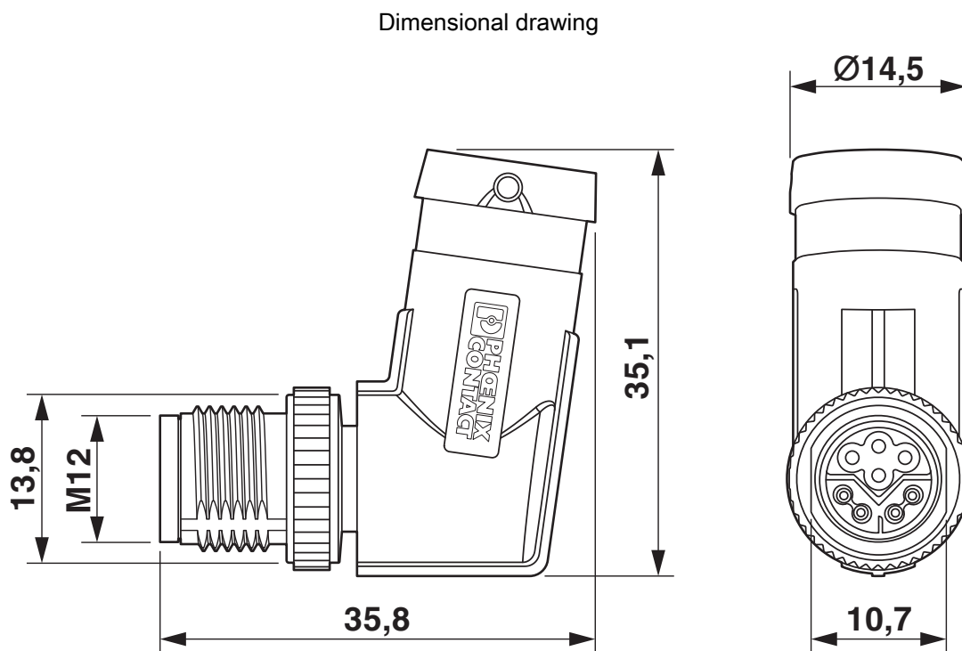
M12 x 1 male plug, angled, shielded
