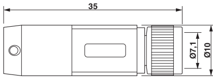
Dimensioned drawing
