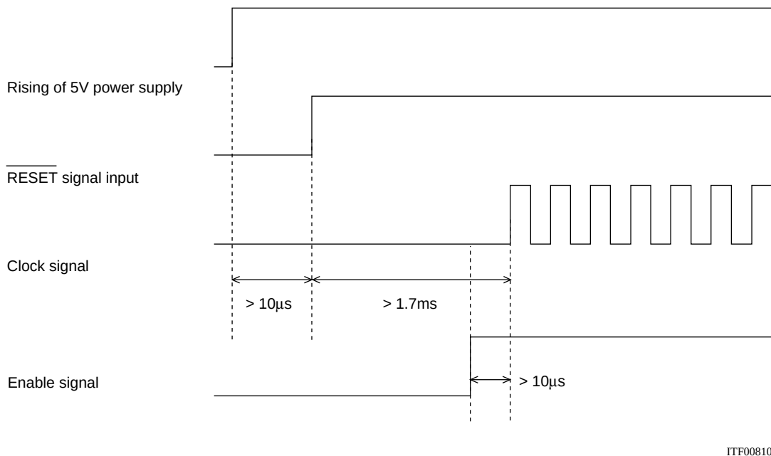
Figure 2. Input timings of RESET signal, Enable signal and Clock signal
