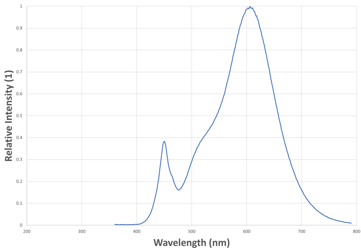
Relative Output vs Wavelength 2700K
