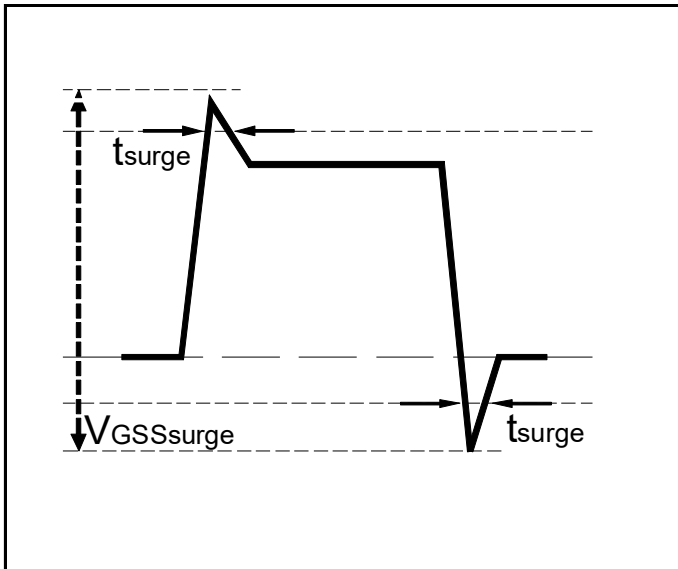
Figure 1. Example of acceptable V GS waveform
