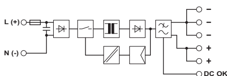
Block diagram
