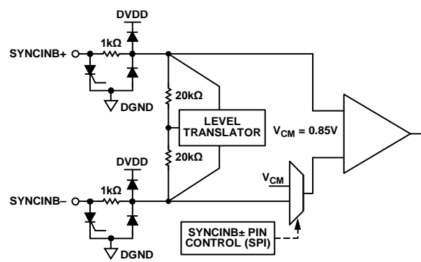
Figure 108. SYNCINB± Inputs
