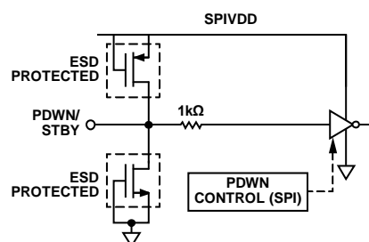
Figure 113. PDWN/STBY Input
