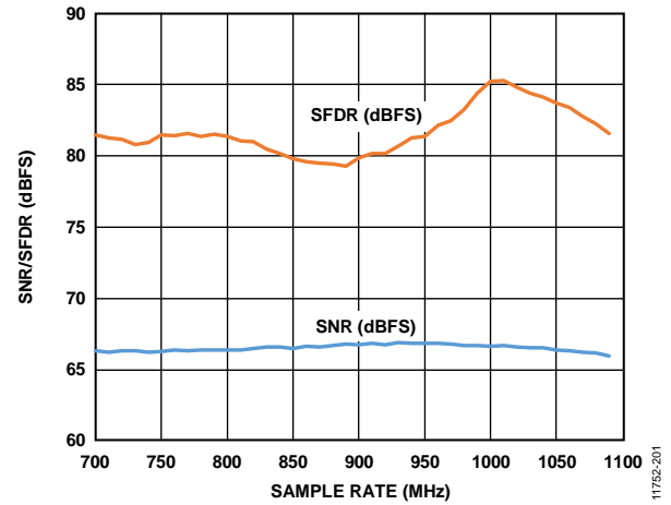
Figure 39. SNR/SFDR vs. f_{IN} , f_{IN} = 170.3 MHz; Buffer Control 1 (0x018) = 3.0x
