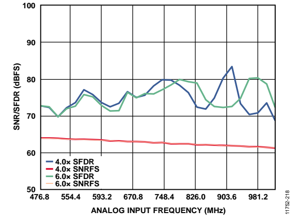
Figure 41. SNR/SFDR vs. f_{IN} ; 500 MHz < f_{IN} < 1 GHz; Buffer Control 1 (0x018) = 4.0x and 6.0x
