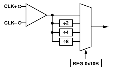
Figure 137. Clock Divider Circuit
