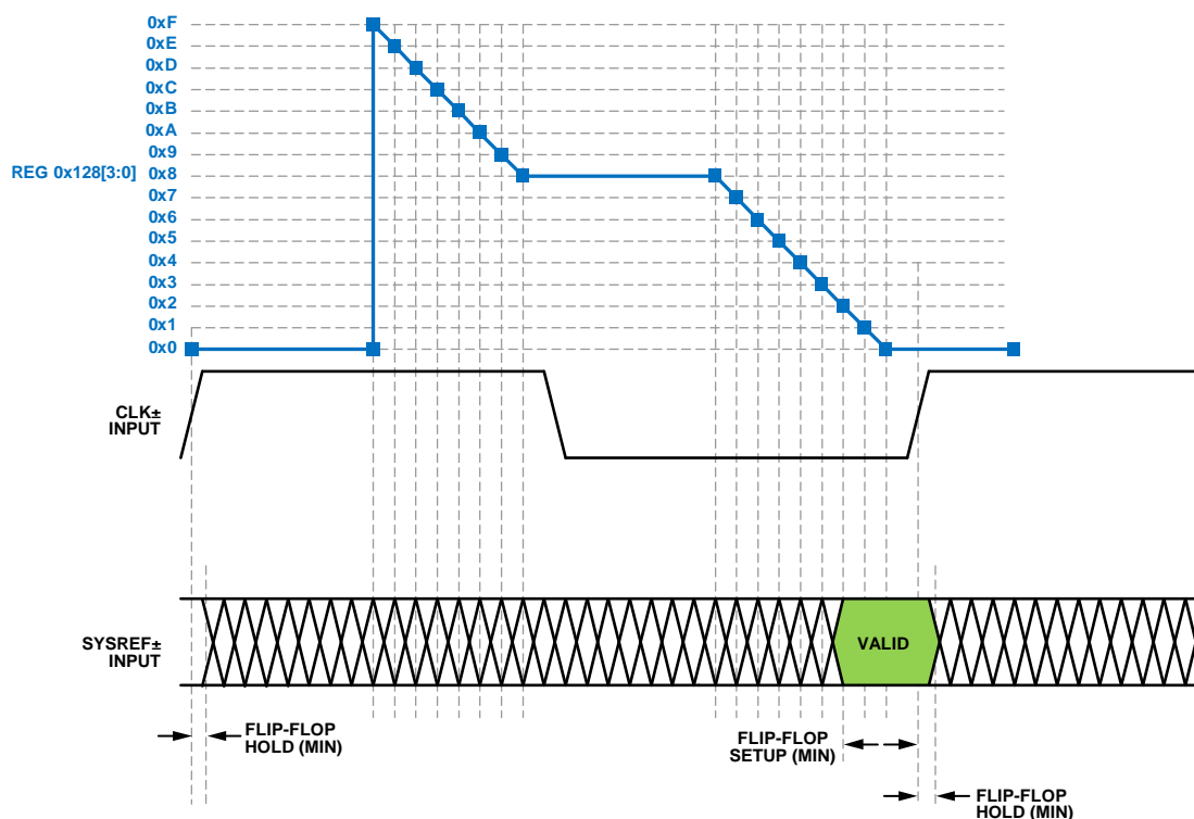
Figure 172. SYSREF± Setup Detector
