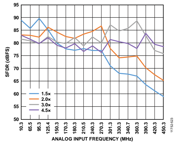
Figure 125. Buffer Current Sweeps, AD9680-820 (SFDR vs. I_{BUFF} ); f_{IN} < 500 MHz; Front-End Network Shown in Figure 115
