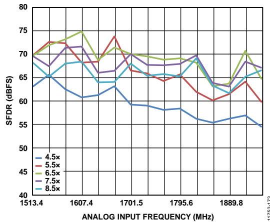
Figure 123. Buffer Current Sweeps, AD9680-1000 (SFDR vs. I_{BUFF} ); 1500 MHz < f_{IN} < 2000 MHz; Front-End Network Shown in Figure 115
