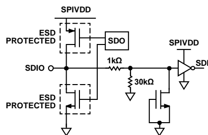
Figure 111. SDIO Input
