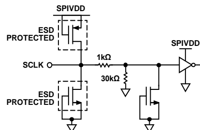
Figure 109. SCLK Input
