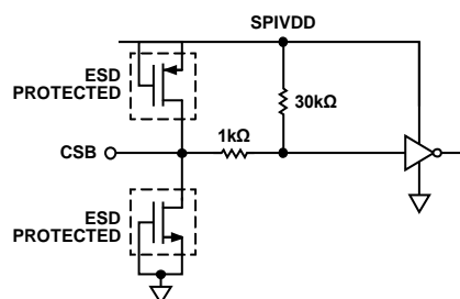
Figure 110. CSB Input
