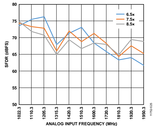
Figure 127. Buffer Current Sweeps, AD9680-820 (SFDR vs. I_{BUFF} ); 1000 MHz < f_{IN} < 2000 MHz; Front-End Network Shown in Figure 115
