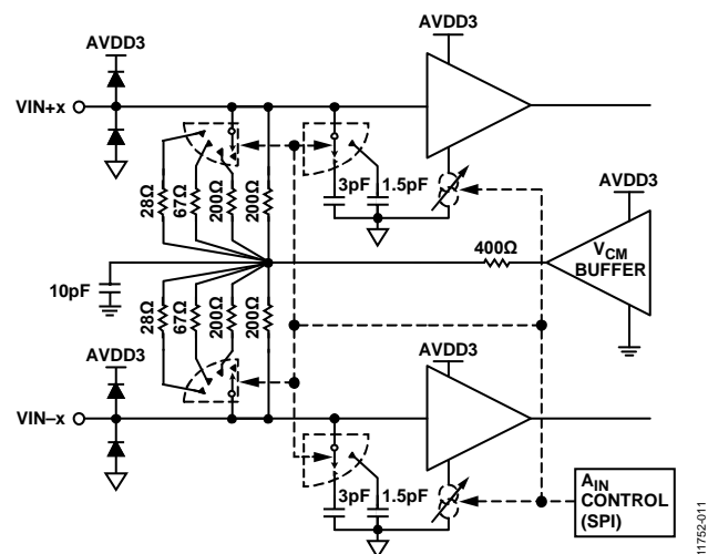
Figure 104. Analog Inputs
