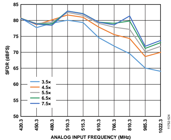
Figure 126. Buffer Current Sweeps, AD9680-820 (SFDR vs. I_{BUFF} ); 500 MHz < f_{IN} < 1000 MHz; Front-End Network Shown in Figure 115
