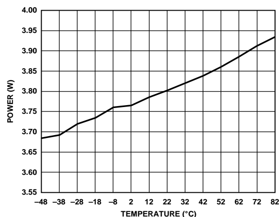
Figure 28. Power Dissipation vs. Temperature
