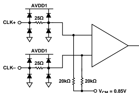
Figure 105. Clock Inputs
