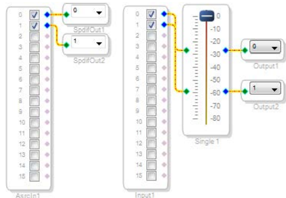
Figure 49. Signal Flow Including S/PDIF Input (via ASRC) and S/PDIF Output
