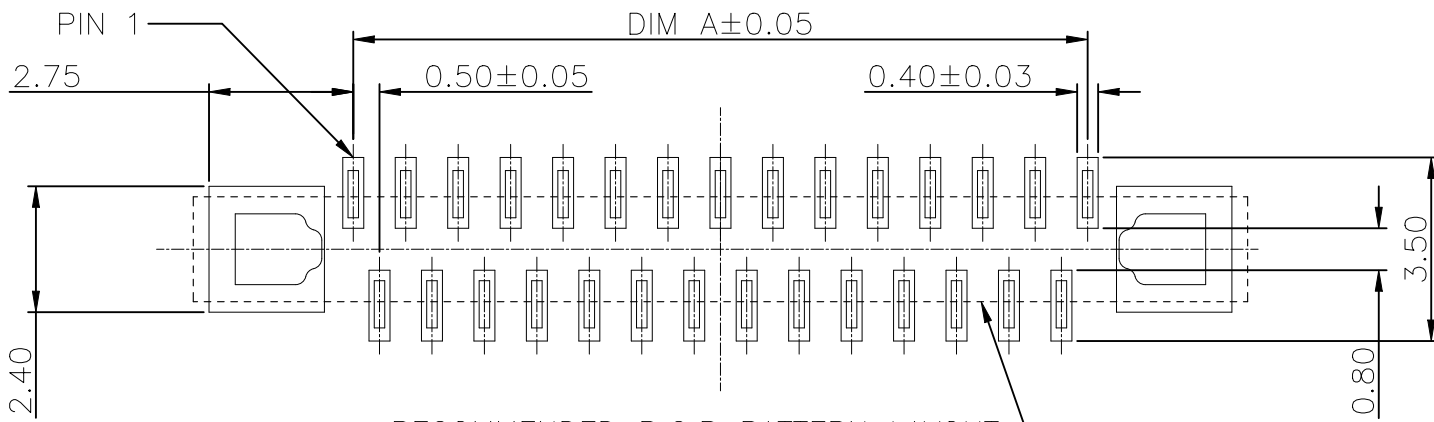
RECOMMENDED P.C.B PATTERN LAYOUT
