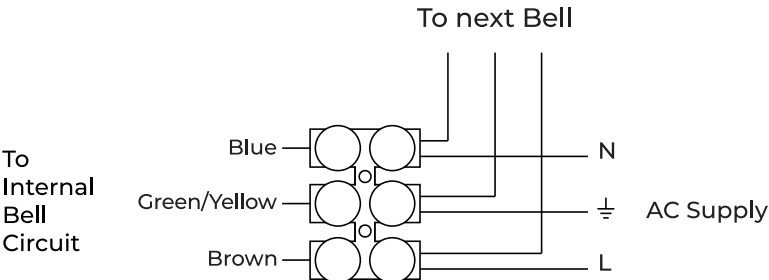
Wiring Diagram 2 (AC)
