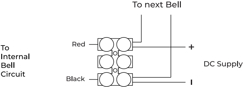
Wiring Diagram 1 (DC)
