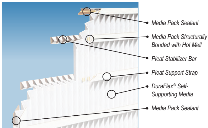
PerfectPleat® SC M7 2" Filter Construction
