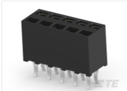
TE Part # 215307-5 2X5P HV100 REC CON. TE, 7.0MM
