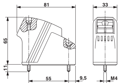
Dimensional drawing
