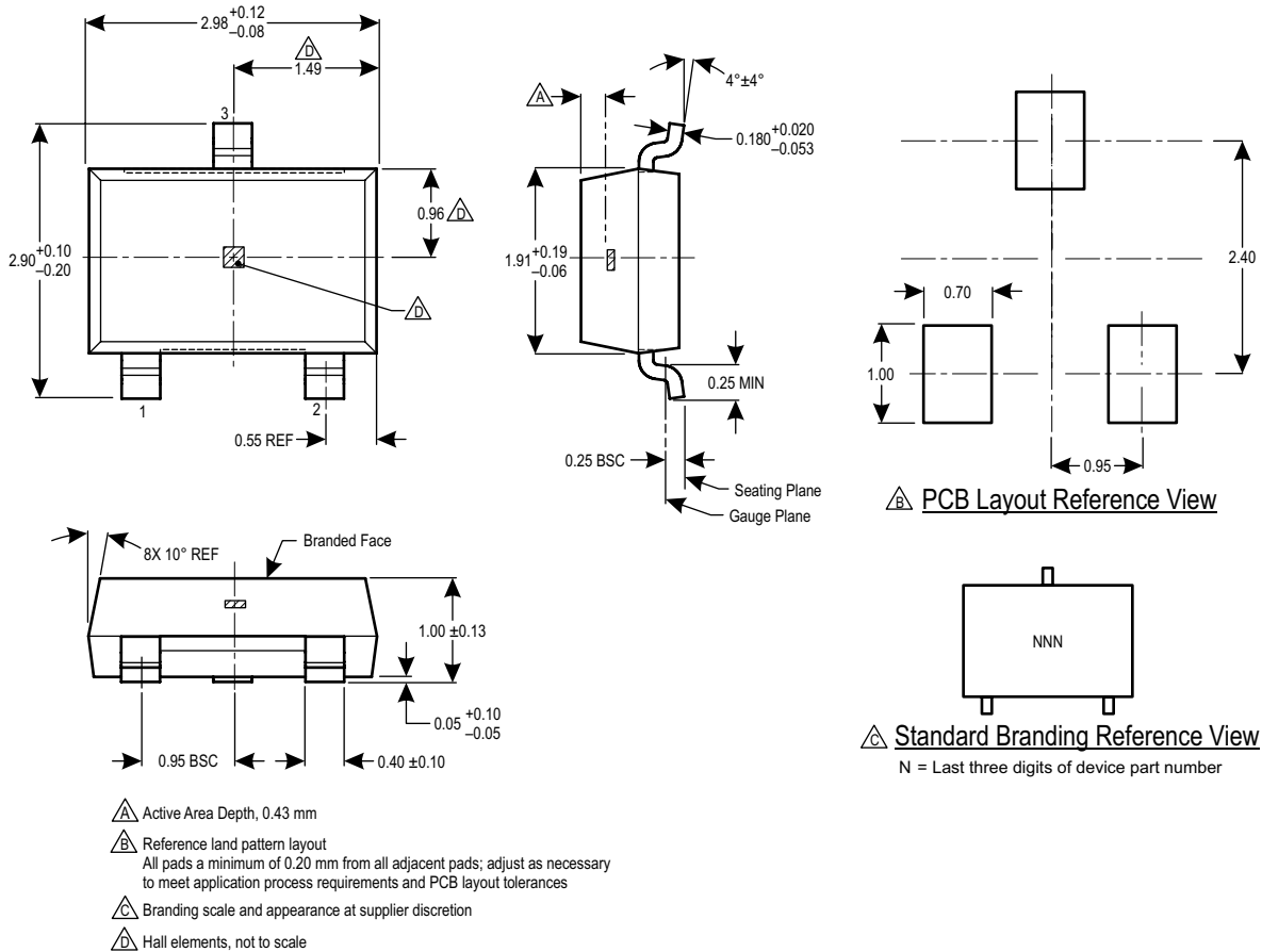
Figure 3: Package LH, 3-Pin SOT-23W
