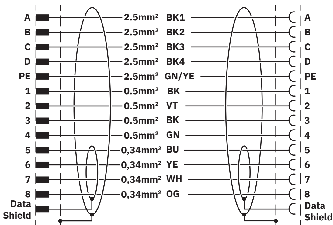
Circuit diagram
