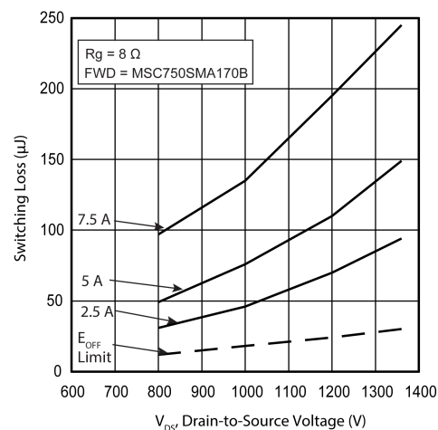
Figure 12 • Switching Energy vs. V_{DS} & I_D
