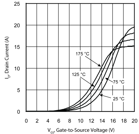
Figure 8 • I_D vs. Gate-to-Source Voltage
