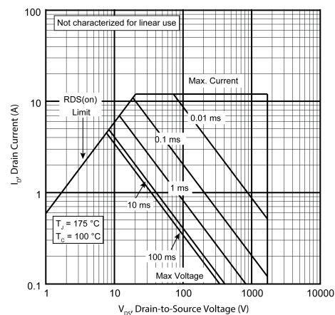
Figure 16 • Forward Safe Operating Area
