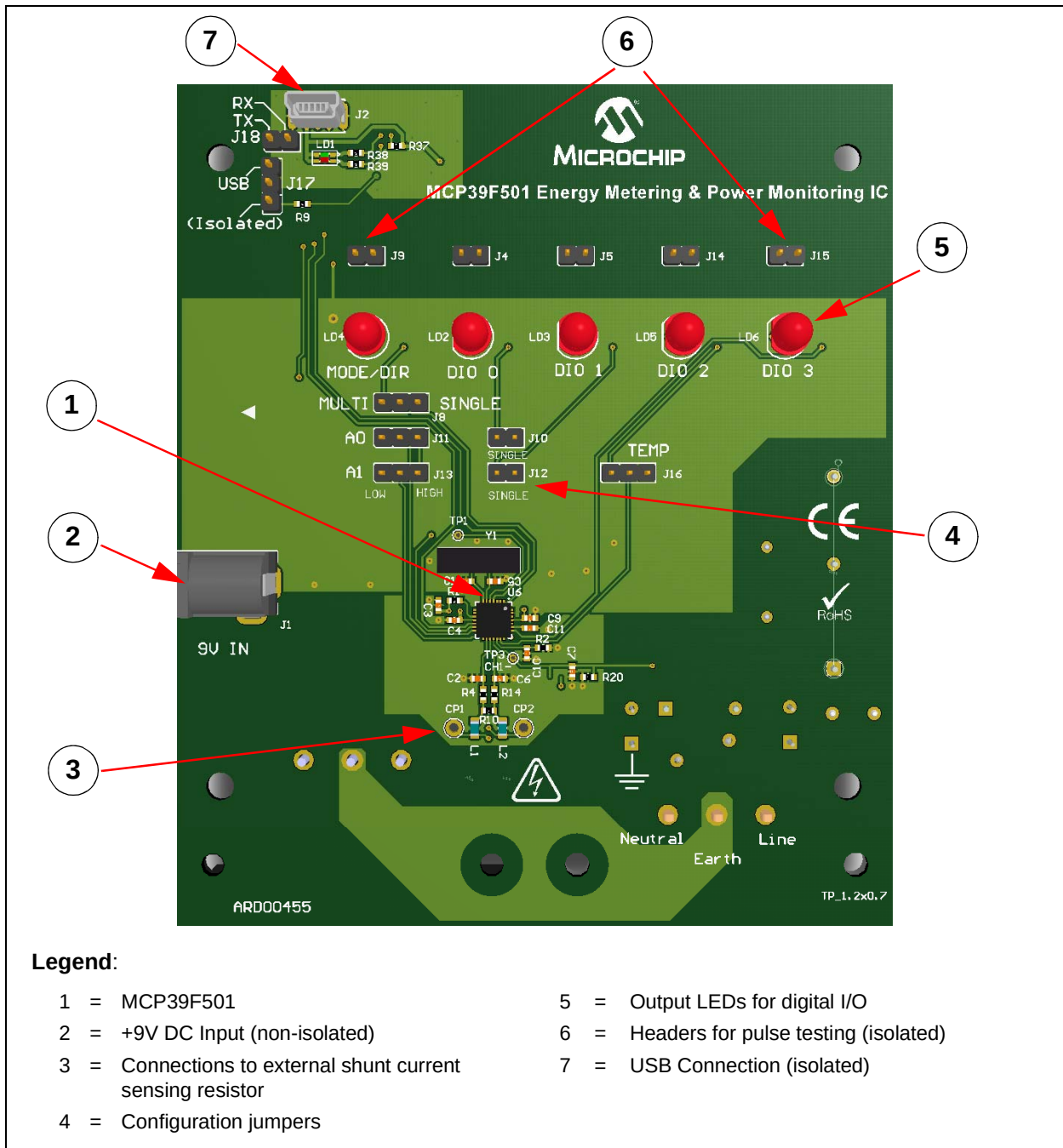
FIGURE 3-1: MCP39F501 Power Monitor Demonstration Board Top View – Hardware Components.
