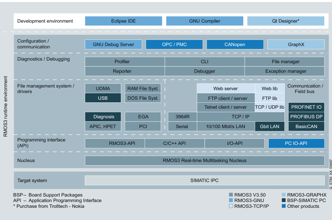
Overview of the RMOS3 operating system structure
