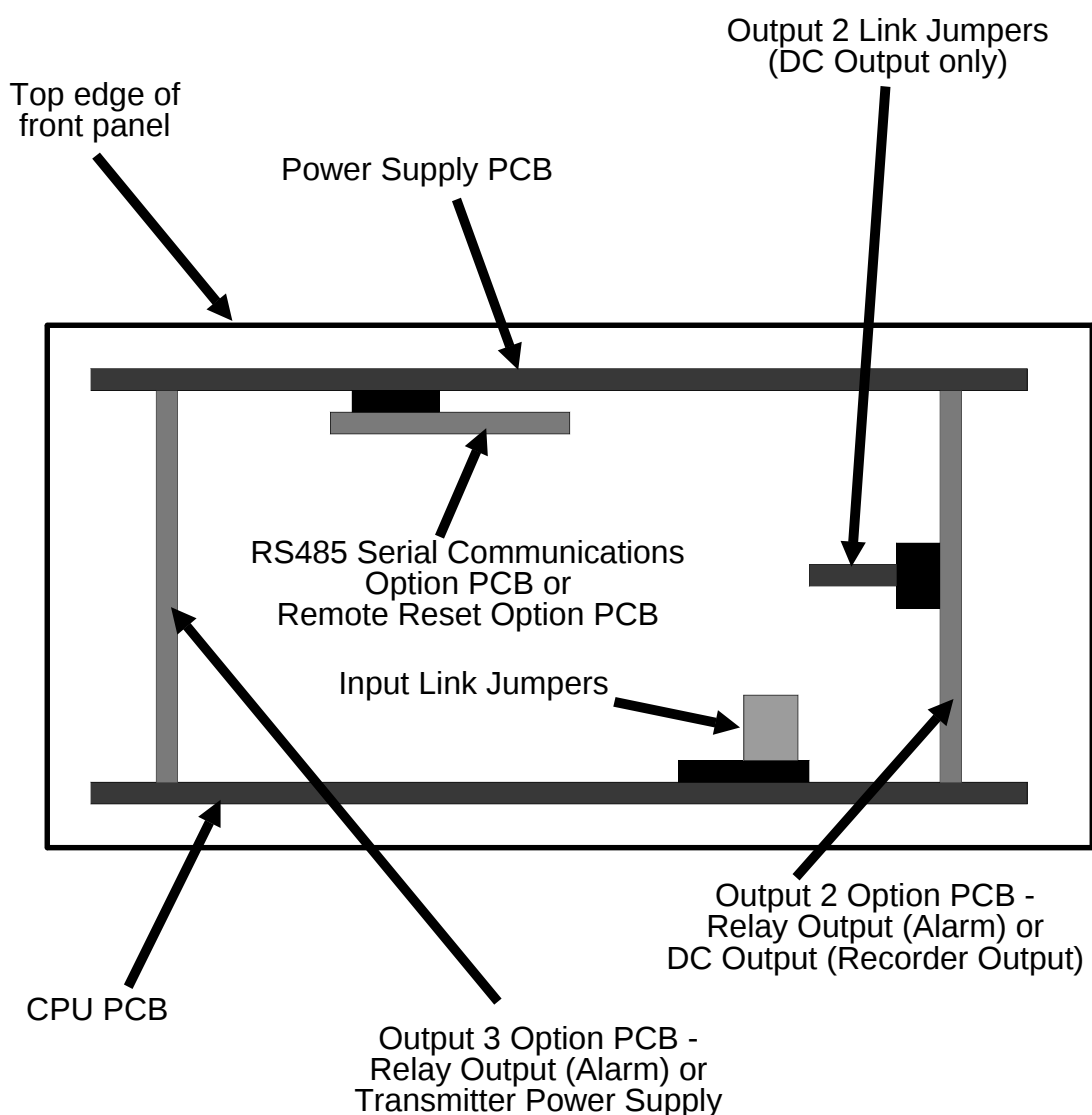
REAR VIEW OF UNHOUSED INSTRUMENT
