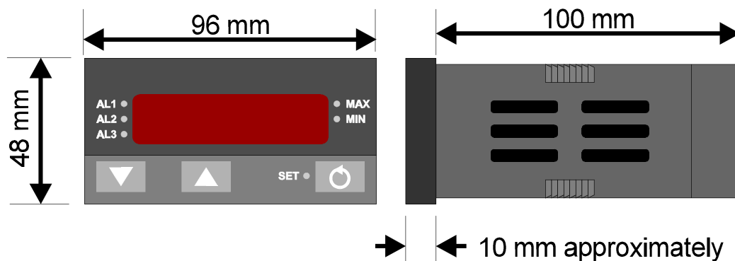
Figure 1-2 Main Dimensions
