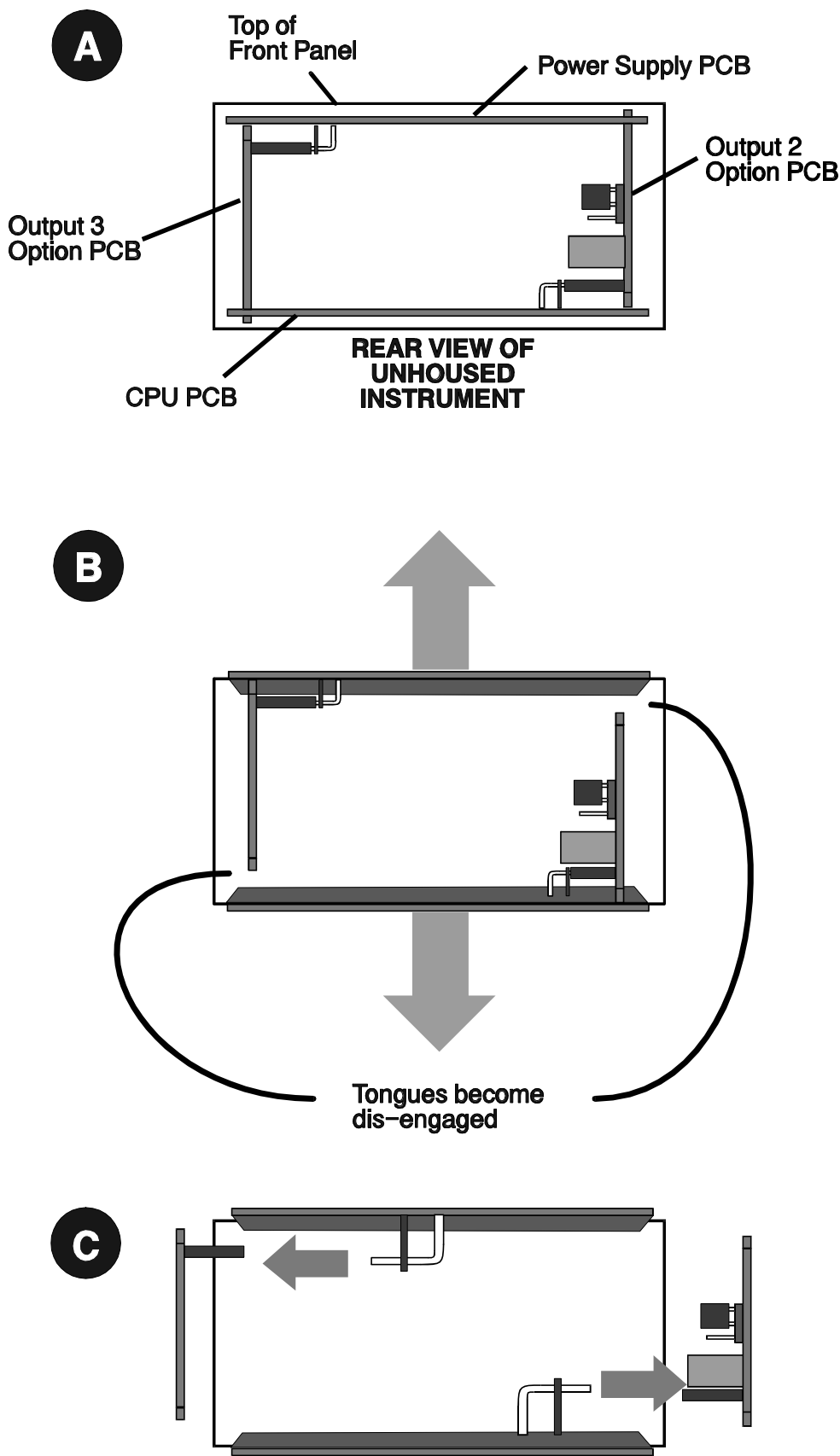
Figure 2-2 Removing the Output 2/Output 3 Option PCBs
