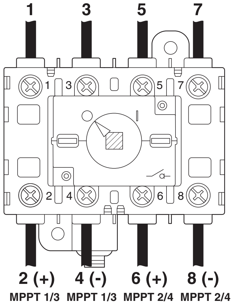
Connection diagram
