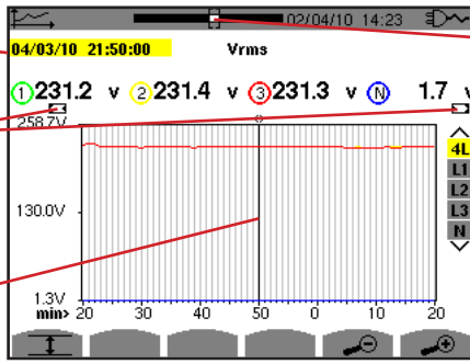
Figura 91: Vrms (4L) sin MIN-AVG-MAX
