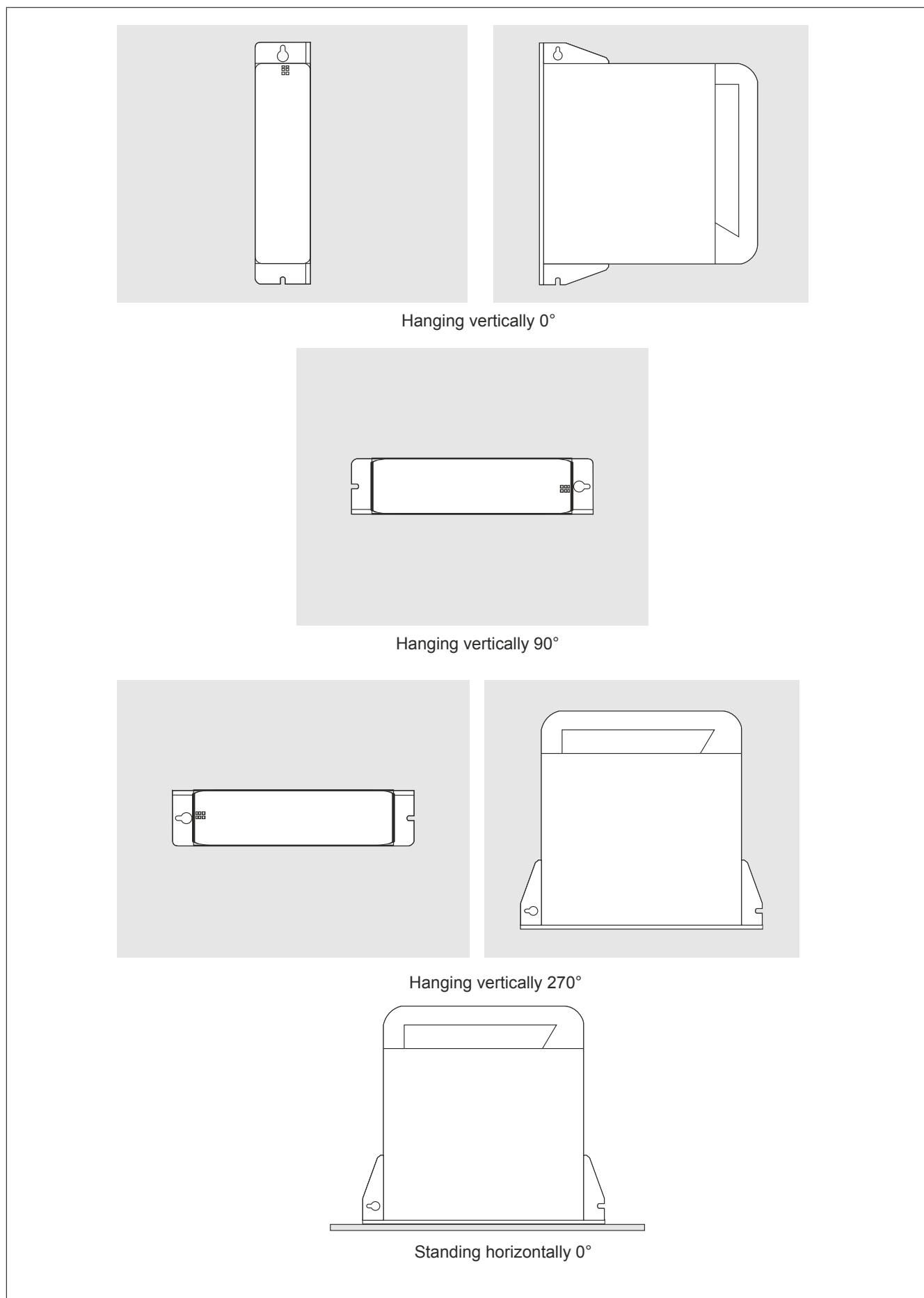
Figure 120: 8EIxXxHWxxx.xxxx-1 / 8EI01xHWSxx.xxxx-1 - Permissible mounting orientations
