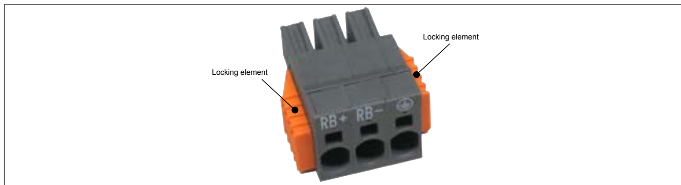
Figure 144: 8TB locking elements (example)
