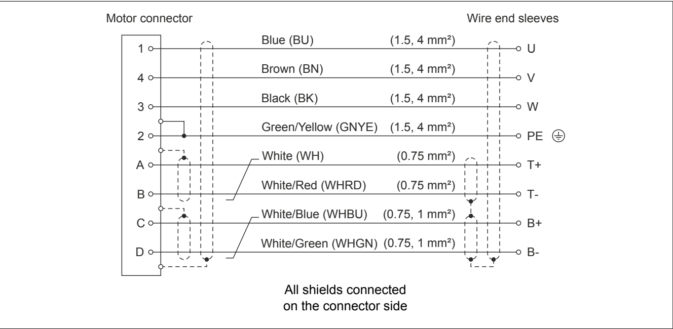
Figure 71: 1.5 mm² - 4 mm² motor cables - Cable diagram
