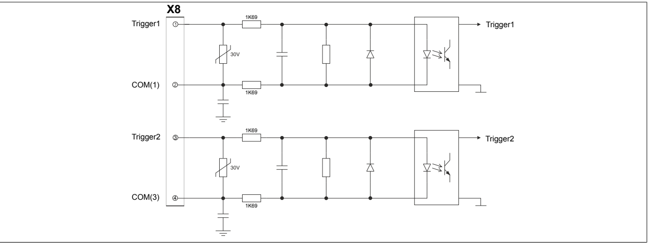
Figure 28: X8 (trigger) - Input/Output circuit diagram
