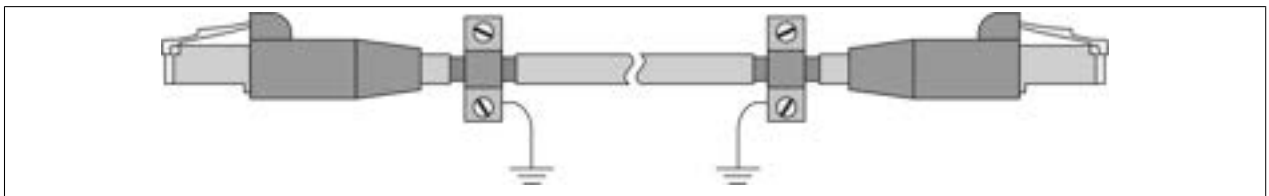
Figure 143: Male RJ45 connector - Grounding the cable shield
