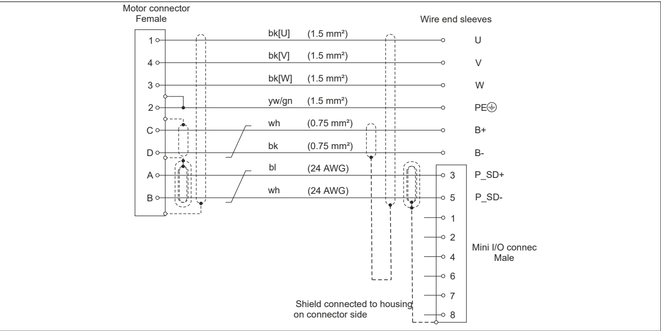
Figure 69: Cable diagram hybrid motor cable EnDat3
