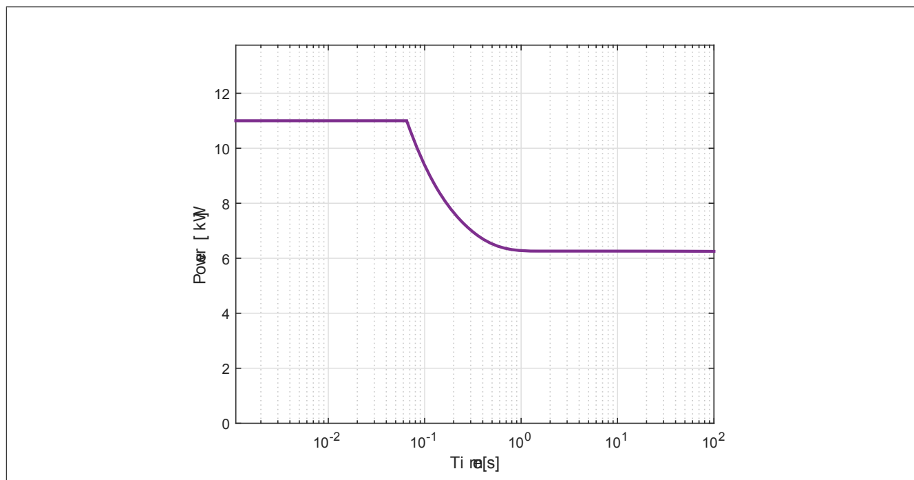
Figure 160: 8EI1X6/2X2/4X5/8X8M... - Peak load capacity
