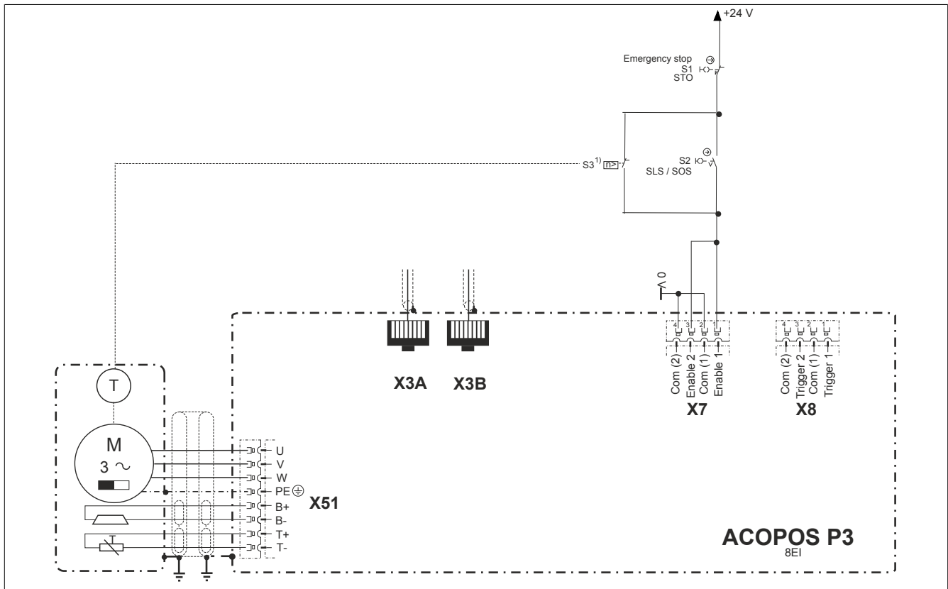
Figure 156: STO, SLS, SOS - Safety category 3 / SIL 2 / PL d
