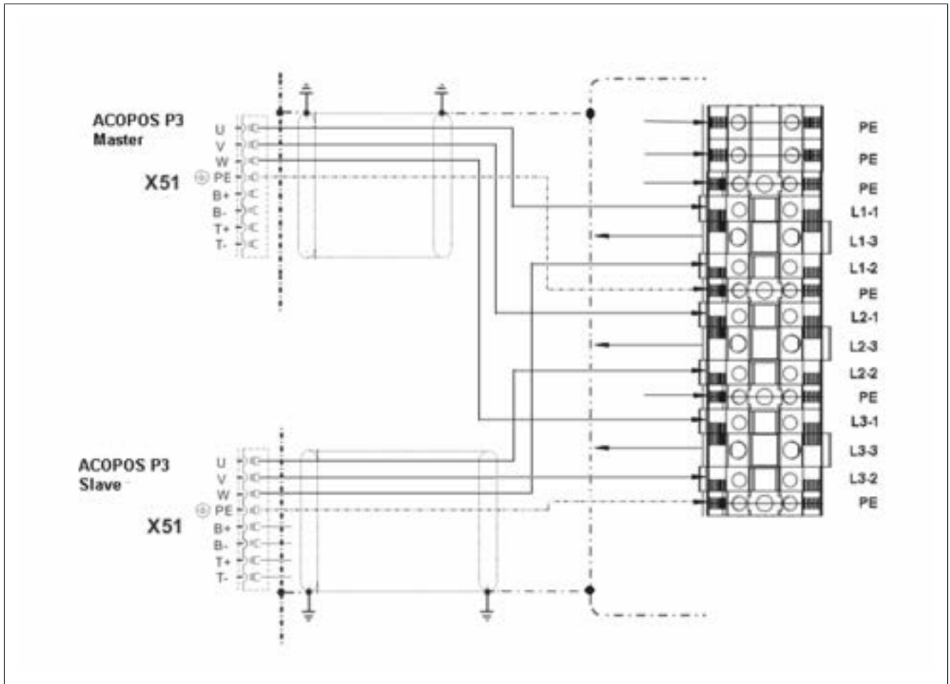
Figure 114: Wiring an ACOPOS P3 to a differential choke
