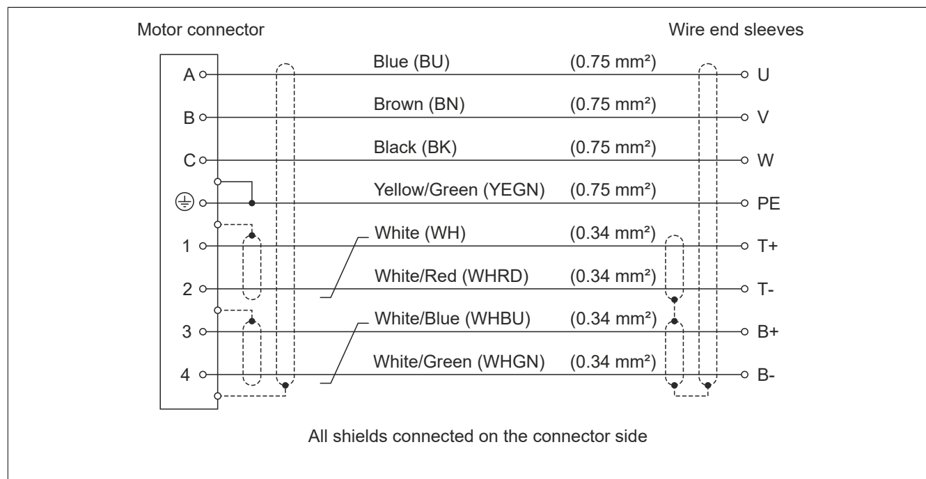
Figure 70: 0.75 mm 2 ESTB motor cables - Cable diagram
