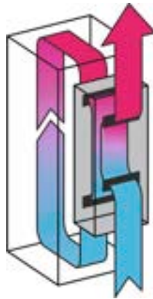
Figure 123: Air/Air heat exchangers - Function diagram
