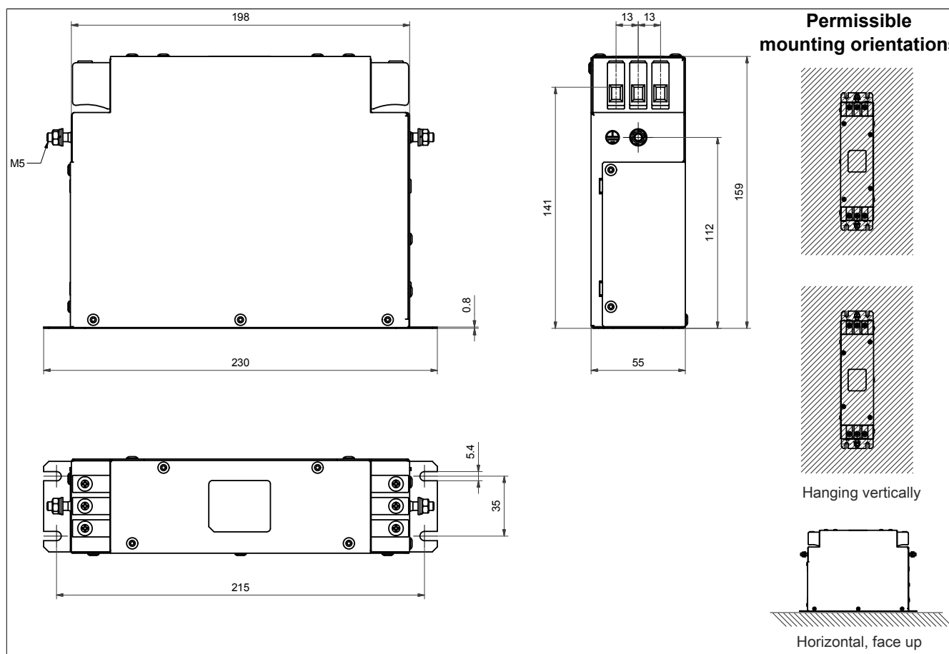
Figure 32: 8EF0160H300.1-1 - Dimension diagram and installation dimensions
