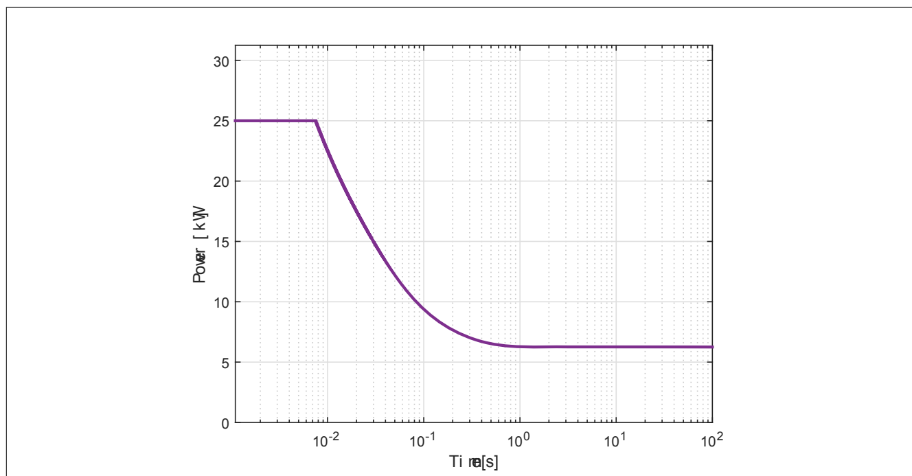
Figure 161: 8EI1X6/2X2/4X5/8X8H... - Peak load capacity
