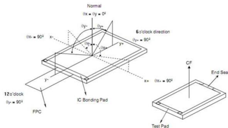
Figure 3. The definition of viewing angle
