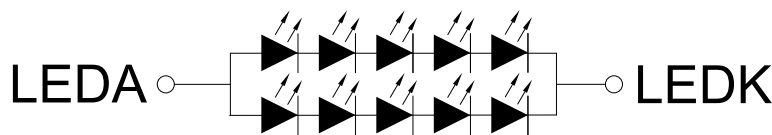
Backlight Circuit Diagram
