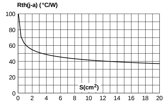
Fig. 11: Thermal resistance junction to ambient versus copper surface under tab (Epoxy printed circuit board FR4, copper thickness: 35\text{ }\mu\text{m} ) (DPAK).
